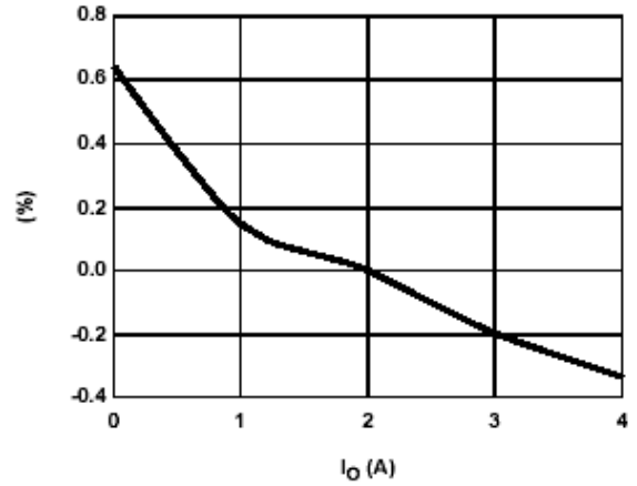
FIGURE 8. LOAD REGULATIONS
