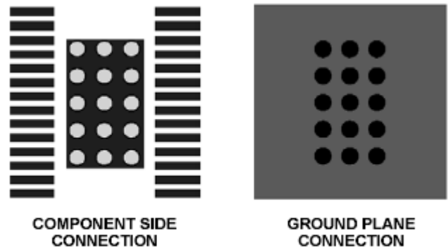
FIGURE 25. PCB LAYOUT - 28-PIN HTSSOP PACKAGE
