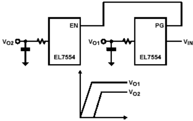
FIGURE 22. CASCADE START-UP
