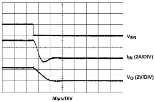
FIGURE 14. SHUT-DOWN
