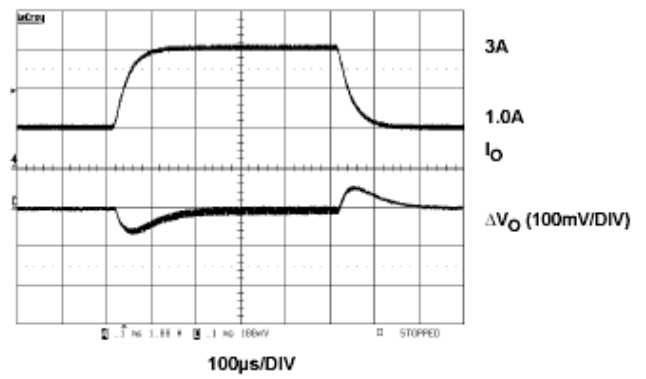
FIGURE 15. TRANSIENT RESPONSE
