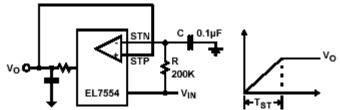
FIGURE 21. ADJUSTABLE START-UP
