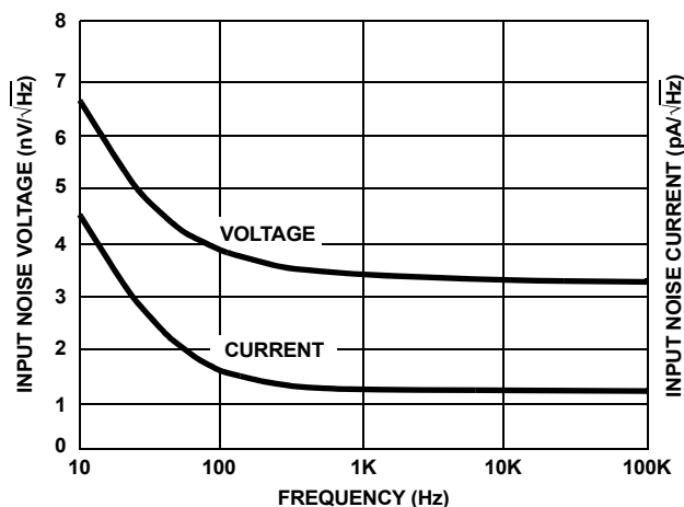
FIGURE 1. NOISE SPECTRUM
