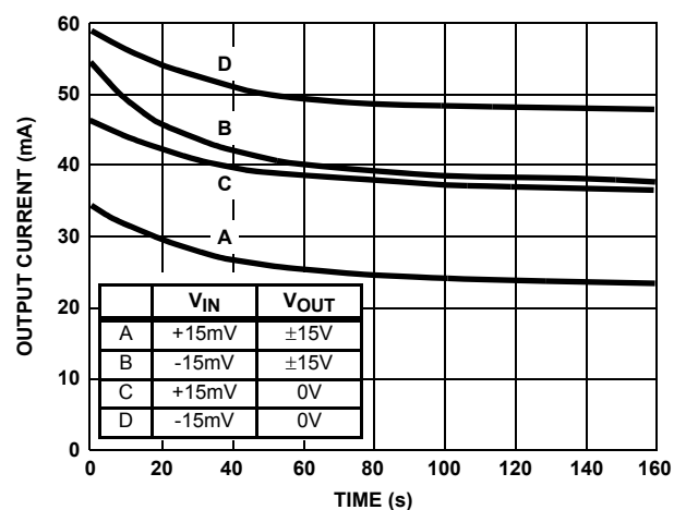
FIGURE 8. SHORT CIRCUIT CURRENT vs TIME
