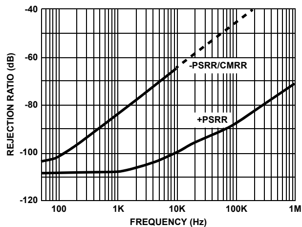
FIGURE 14. REJECTION RATIOS vs FREQUENCY
