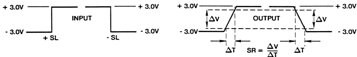
SLEW RATE WAVEFORMS
