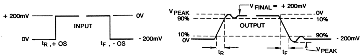
OVERSHOOT, RISE/FALL TIME WAVEFORMS
