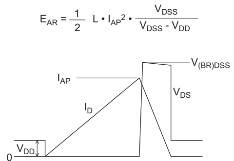
Avalanche Waveform
