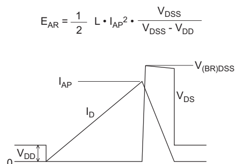
Avalanche Waveform
