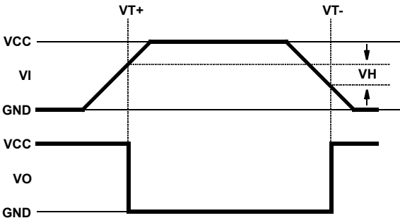
HYSTERESIS DEFINITION
