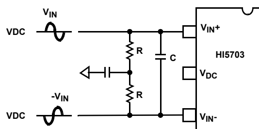
FIGURE 17. DC COUPLED DIFFERENTIAL INPUT
