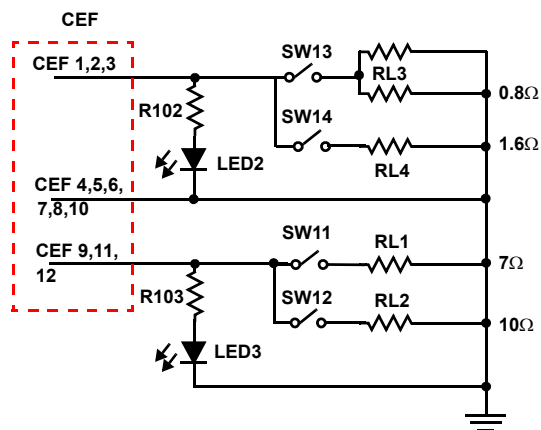
LOAD BOARD
