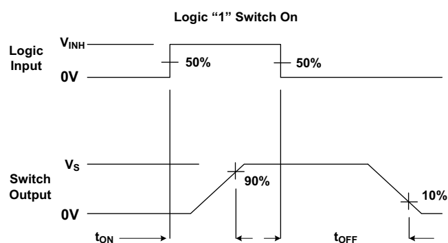
Figure 5. Switching Test Circuit Waveform
