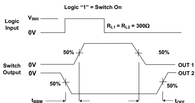
Figure 7. Break-Before-Make Test Circuit Waveforms
