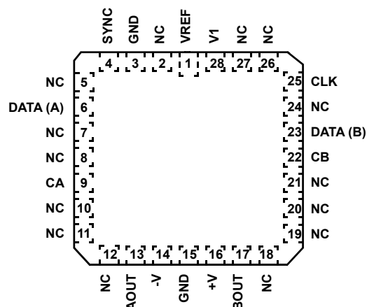
HS-3182 (28 LD CLCC) TOP VIEW
