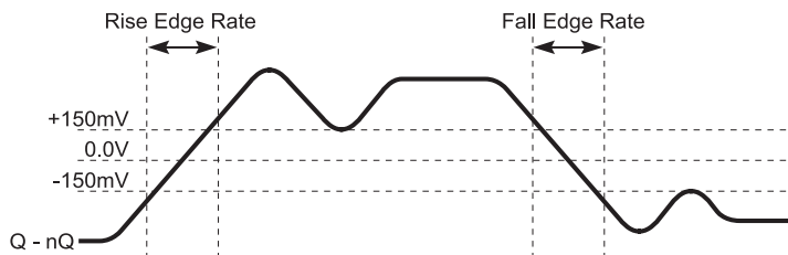
DIFFERENTIAL HCSL MEASUREMENT POINTS FOR RISE/FALL EDGE RATE
