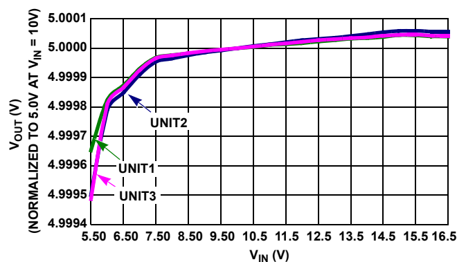
FIGURE 32. LINE REGULATION
