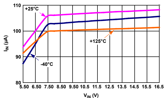
FIGURE 31. I_{IN} vs V_{IN} , 3 TEMPERATURES
