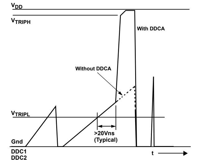
FIGURE 10. NOISE SUPPRESSION. BOOST CURRENT APPLIED WHEN INPUT SIGNAL EXCEEDS 20Vns (TYPICAL)
