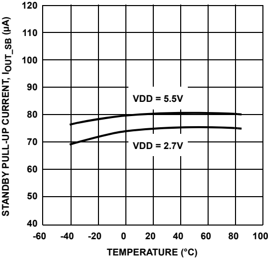
FIGURE 3. STANDBY PULL-UP CURRENT, DDC1, 2 = V DD - 0.5V
