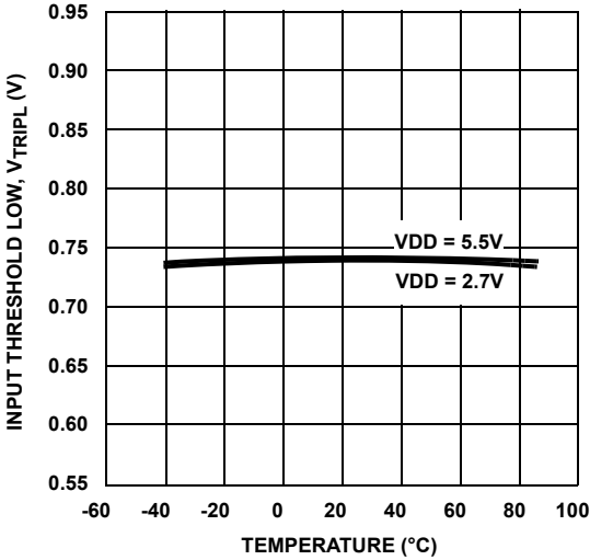
FIGURE 4. V TRIPL VOLTAGE
