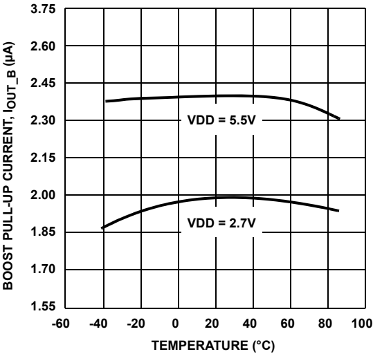
FIGURE 2. BOOST PULL-UP CURRENT, DDC PIN = V DD /2
