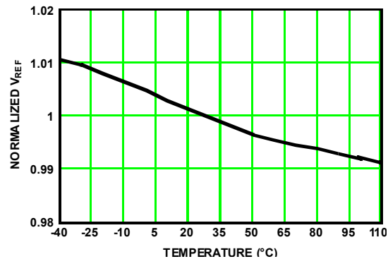
FIGURE 1 REFERENCE VOLTAGE vs. TEMPERATURE
