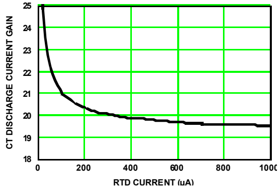
FIGURE 2 CT DISCHARGE CURRENT GAIN vs RTD CURRENT
