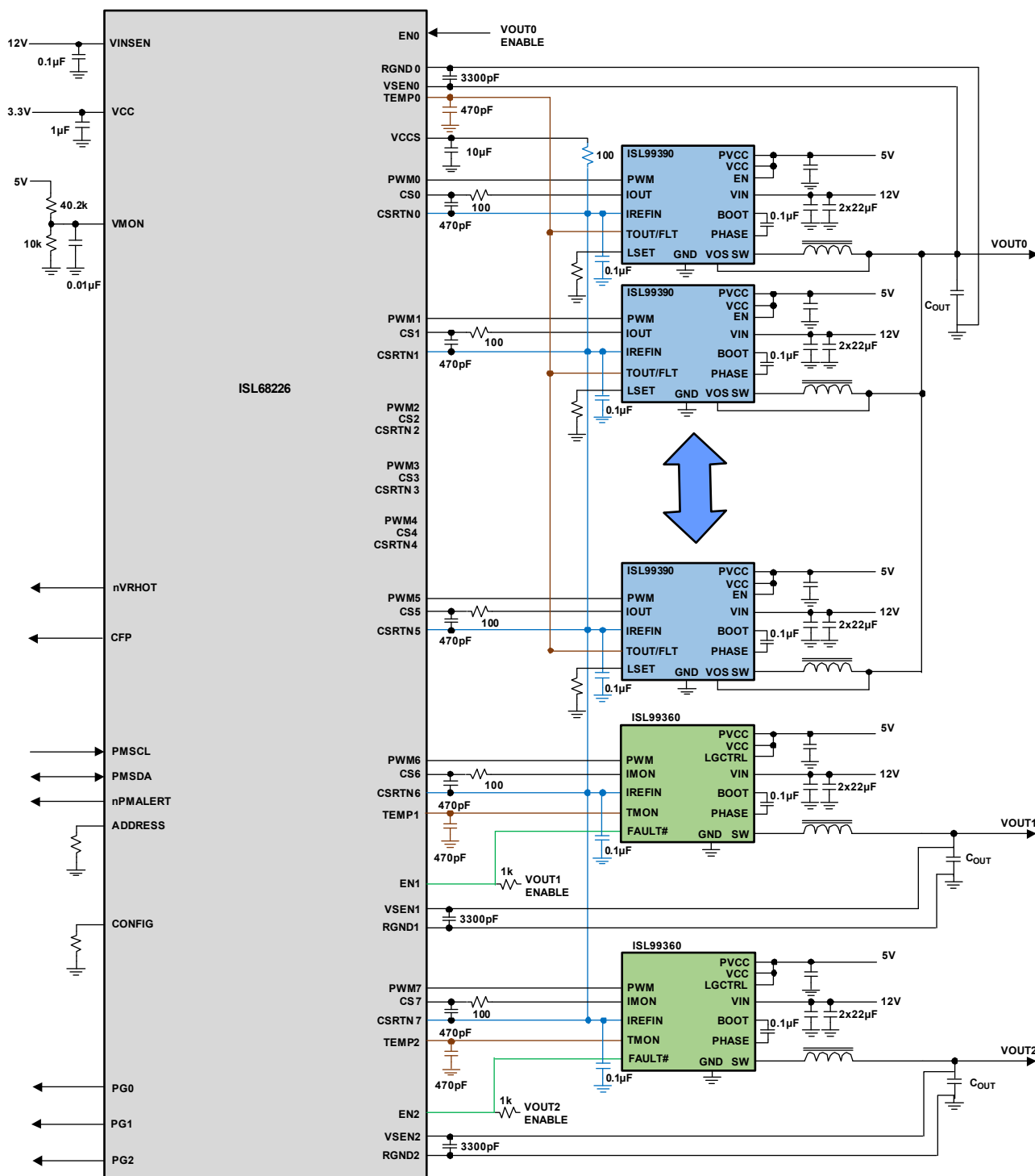
Figure 1. 6+1+1 Solution Using Smart Power Stage
