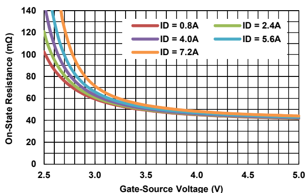
Figure 2. On-State Resistance (+25°C)
