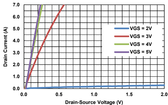
Figure 5. Output Characteristics ( -55^\circ C )
