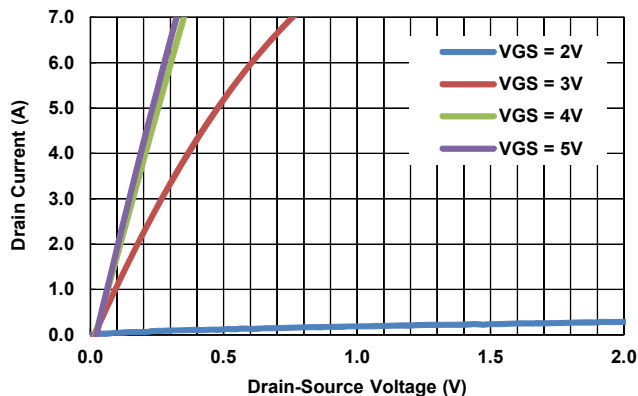
Figure 3. Output Characteristics ( +25^\circ C )
