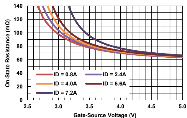
Figure 8. On-State Resistance ( +125^\circ C )
