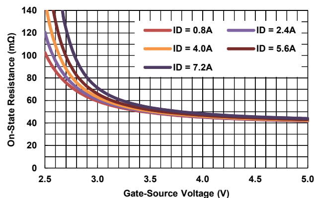
Figure 7. On-State Resistance ( +25^\circ C )
