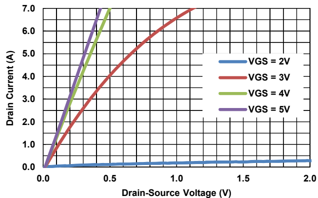
Figure 4. Output Characteristics ( +125^\circ C )
