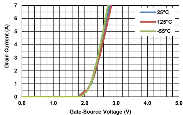
Figure 6. Transfer Characteristics
