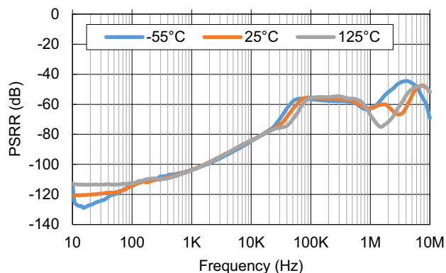
Figure 38. PSRR vs Frequency, V_+ = 2.7V , V_{CM} = 12V
