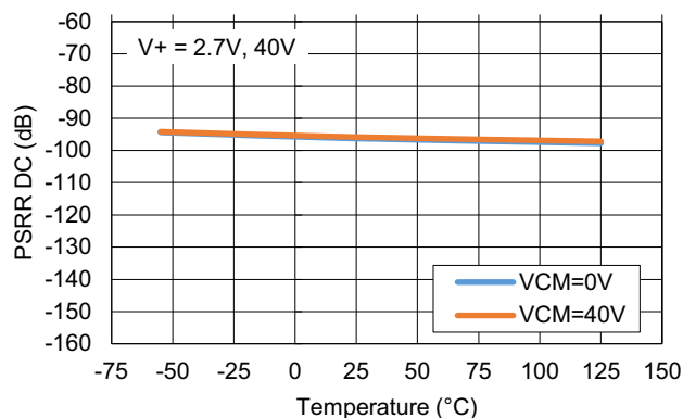
Figure 37. PSRR DC
