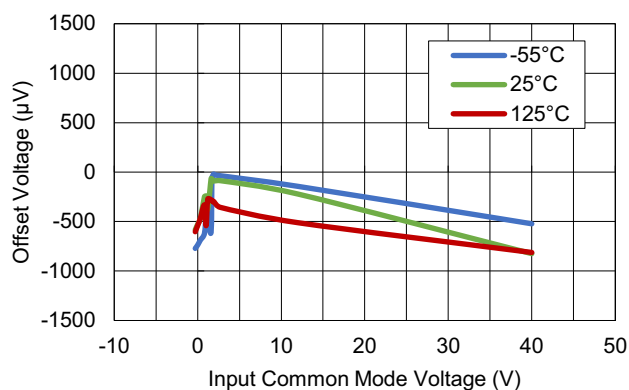
Figure 8. Common-Mode Voltage vs V_{OS} , V_+ = 40V
