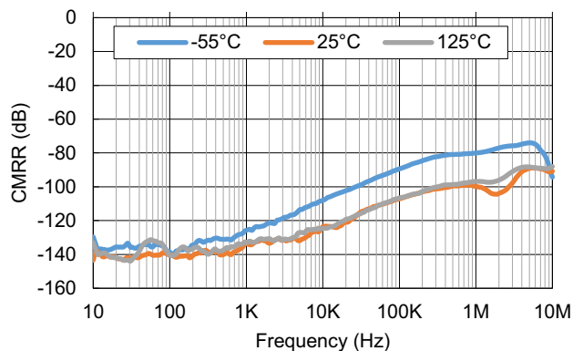
Figure 36. CMRR vs Frequency, V_+ = 12V , V_{CM} = 40V
