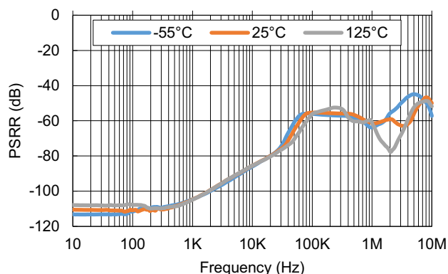
Figure 40. PSRR vs Frequency, V_+ = 40V , V_{CM} = 12V
