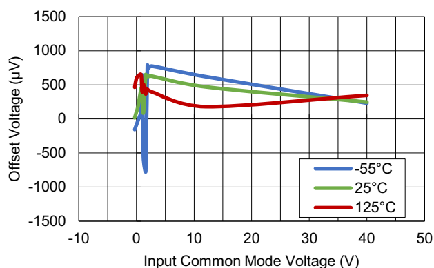
Figure 10. Common-Mode Voltage vs V_{OS} , V_+ = 2.7V
