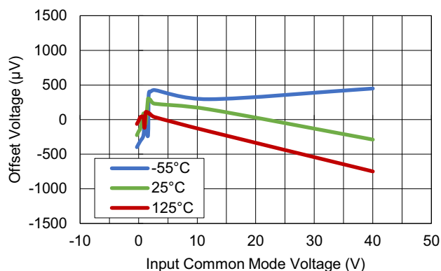
Figure 6. Common-Mode Voltage vs V_{OS} , V_+ = 12V
