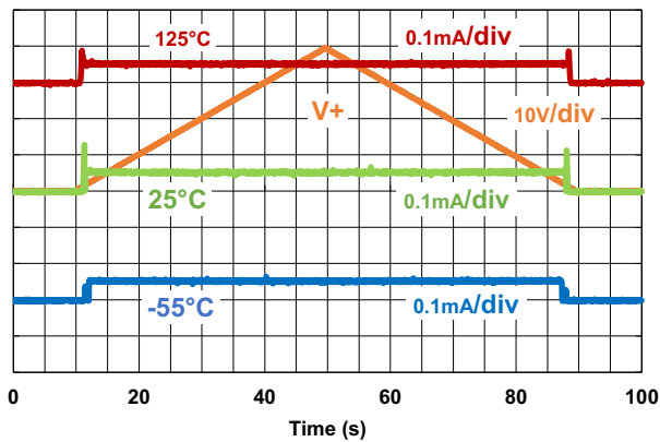
Figure 25. Power Supply Ramp at 1V/s
