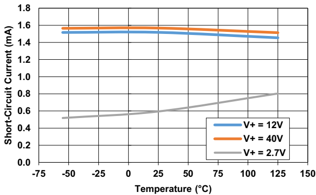
Figure 41. Short-Circuit Current
