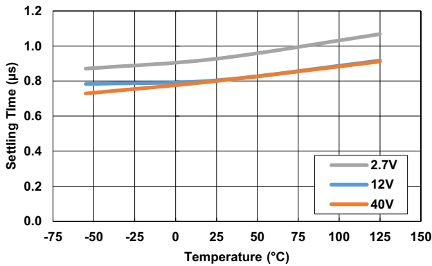
Figure 23. Settling Time
