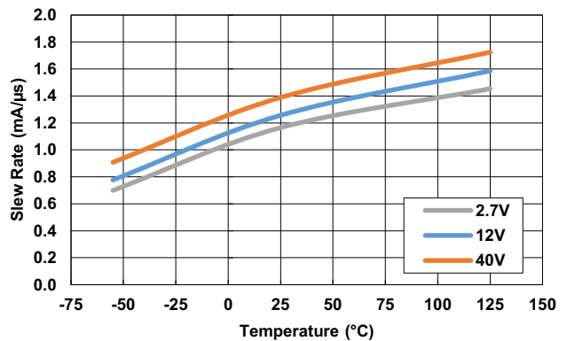
Figure 20. Slew Rate
