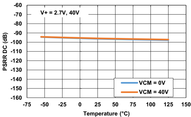
Figure 37. PSRR DC
