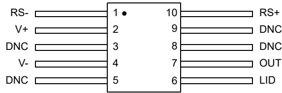
Figure 4. Pin Assignments - Top View
