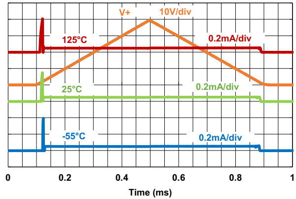
Figure 26. Power Supply Ramp at 1V/10µs
