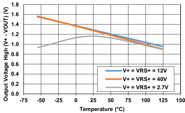
Figure 43. Output Voltage High (Referred to V_+ )
