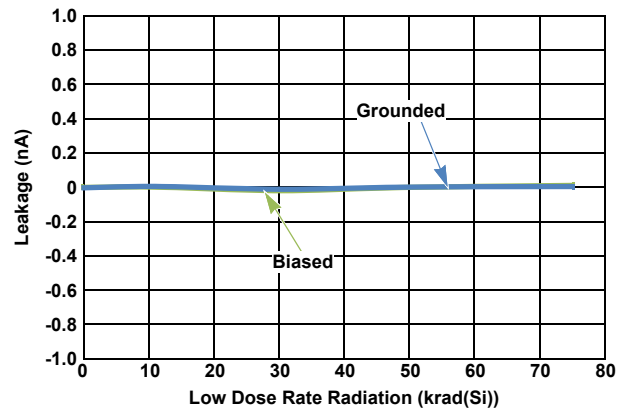
Figure 50. I_{S(OFF)} ( V^+ = 3.6\text{V} , V_{IN} = 3.1\text{V} )
