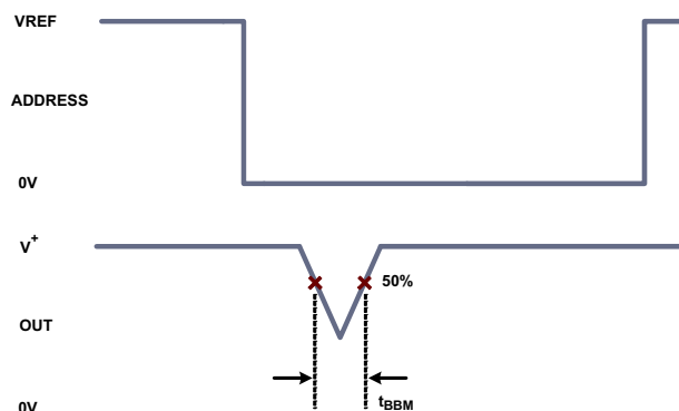
Figure 10. Break-Before-Make Diagram
