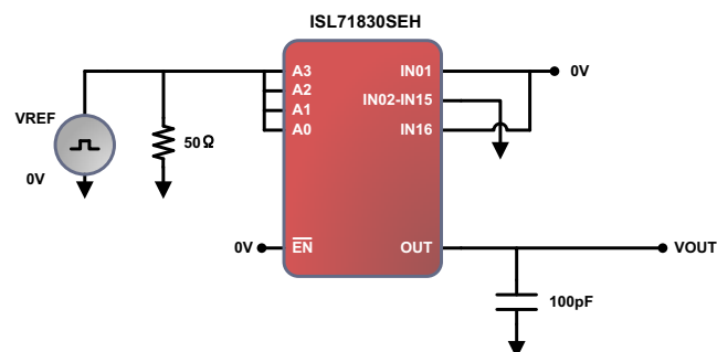
Figure 11. Charge Injection Test Circuit
