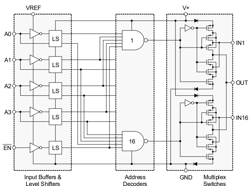
Figure 56. ISL71830SEH Inner Structure
