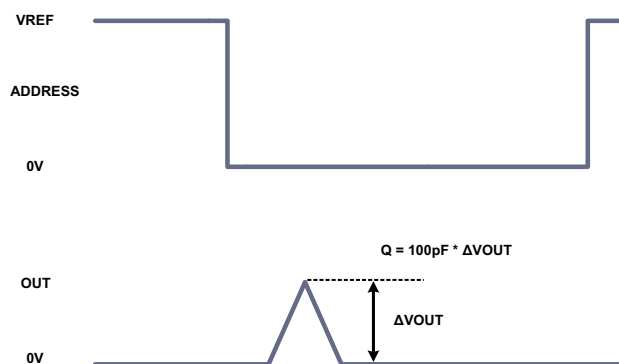
Figure 12. Charge Injection Diagram
