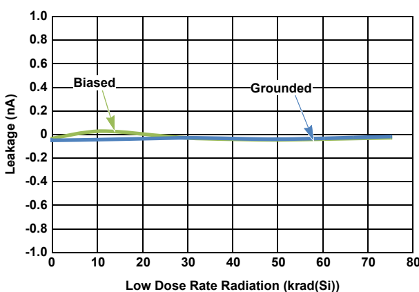
Figure 53. I_{D(ON)} ( V^+ = 3.6\text{V} , V_{IN} = 3.1\text{V} )
