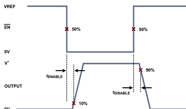
Figure 8. Time to Enable/Disable Output Diagram
