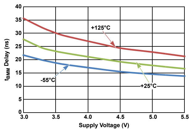
Figure 22. Break-Before-Make Delay
