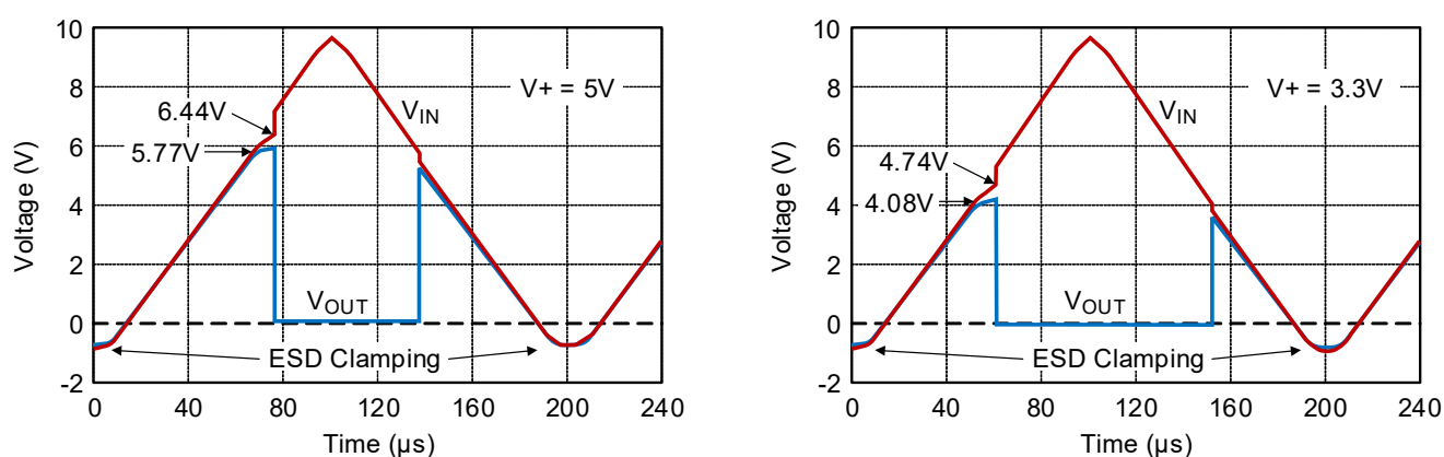
Figure 55. Overvoltage Protection Thresholds at 5V and 3.3V Supply
