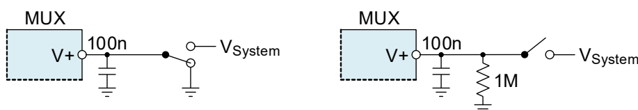
Figure 57. Cold Sparing Setup with Grounded and Floating Supplies
