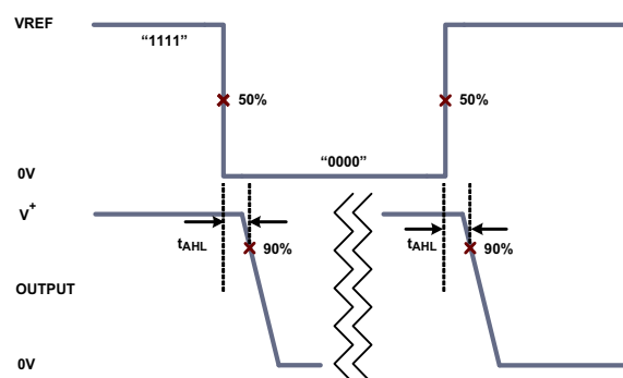
Figure 6. Address Time to Output Diagram
