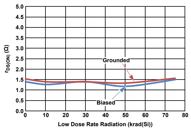
Figure 48. r_{DS(ON)} Match ( V^+ = 3V , V_{IN} = 0.5V )
