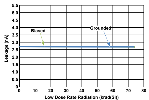
Figure 52. I_{S(ON)} ( V^+ = 3.6\text{V} , V_{IN} = 7\text{V} )
