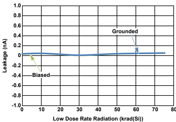
Figure 51. I_{S(OFF)} ( V^+ = 3.6\text{V} , V_{IN} = 7\text{V} )
