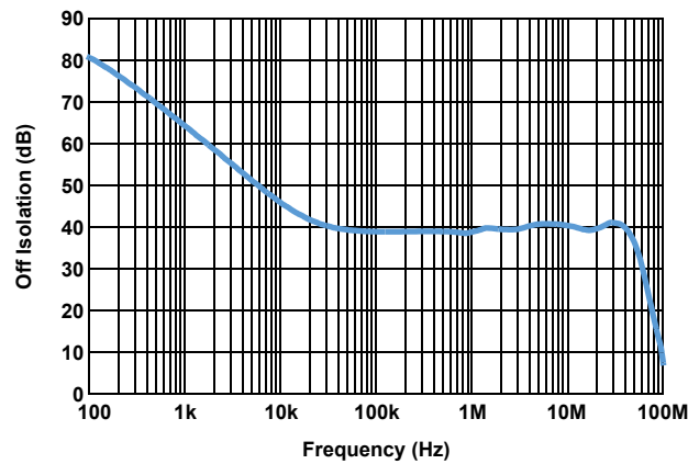
Figure 28. Off Isolation ( V^+ = 5V , +25^\circ\text{C} , R_L = \text{OPEN} )
