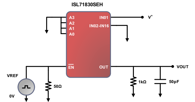
Figure 7. Time to Enable/Disable Output Test Circuit
