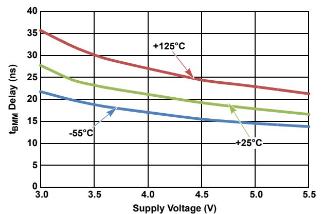
Figure 22. Break-Before-Make Delay
