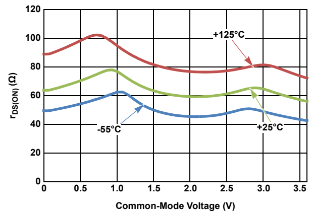
Figure 18. r_{DS(ON)} vs Common-Mode Voltage ( V^+ = 3.6V )
