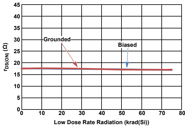
Figure 35. r_{DS(ON)} Flatness ( V^+ = 4.5V )
