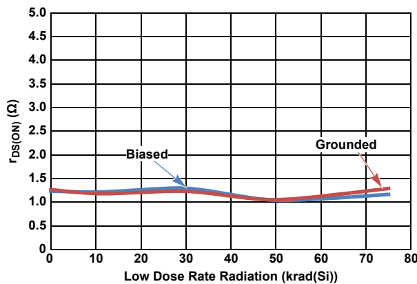
Figure 49. r_{DS(ON)} Match ( V^+ = 3\text{V} , V_{IN} = 2.5\text{V} )
