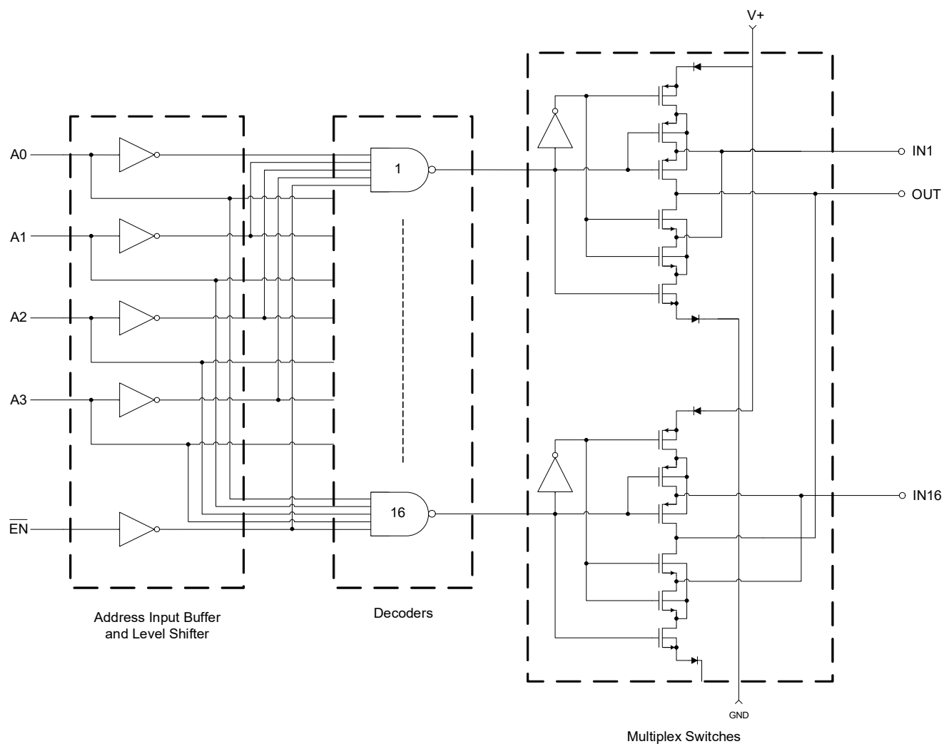
Figure 3. Block Diagram
