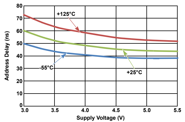
Figure 20. Address Propagation Delay (Low to High)
