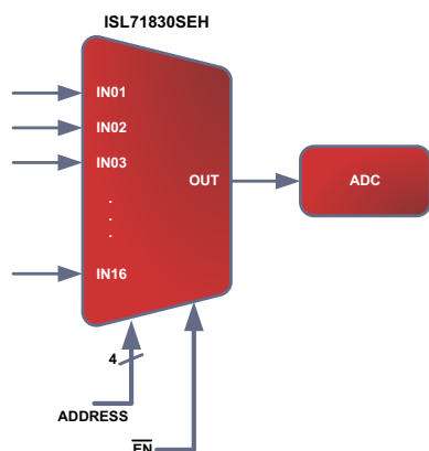
Figure 1. Typical Application
