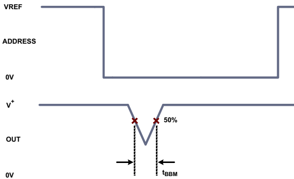
Figure 10. Break-Before-Make Diagram
