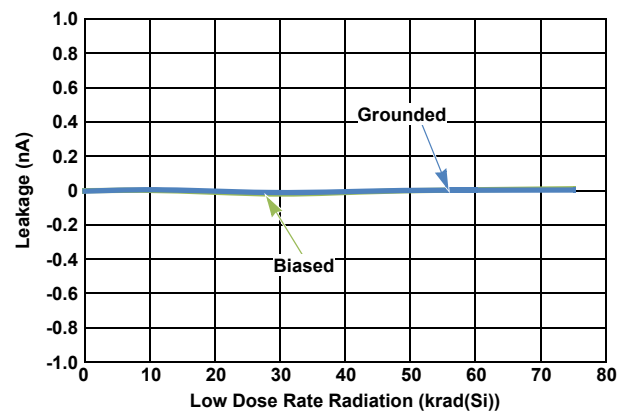
Figure 50. I_{S(OFF)} ( V^+ = 3.6\text{V} , V_{IN} = 3.1\text{V} )
