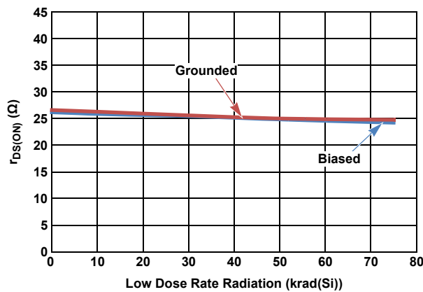
Figure 47. r_{DS(ON)} Flatness ( V^+ = 3\text{V} )
