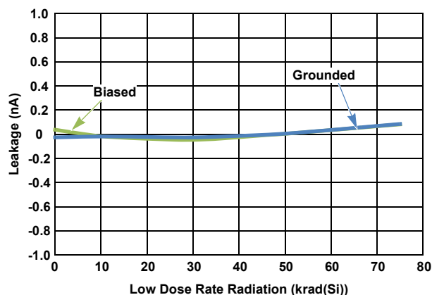
Figure 54. I_{D(OFF)} ( V^+ = 3.6\text{V} , V_{IN} = 3.1\text{V} )
