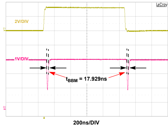
Figure 23. Break-Before-Make Delay
