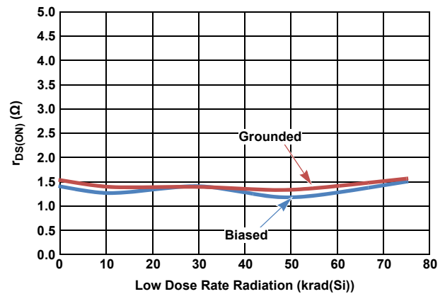
Figure 48. r_{DS(ON)} Match ( V^+ = 3\text{V} , V_{IN} = 0.5\text{V} )
