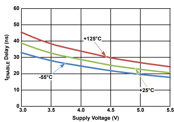
Figure 24. Enable to Output Propagation Delay
