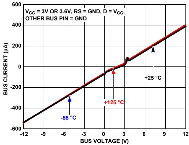
Figure 30. Bus Pin Leakage vs \pm 12V_{CM}
