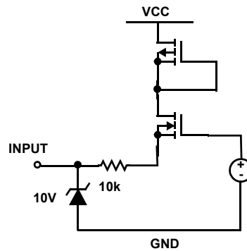
Figure 8. RS Input
