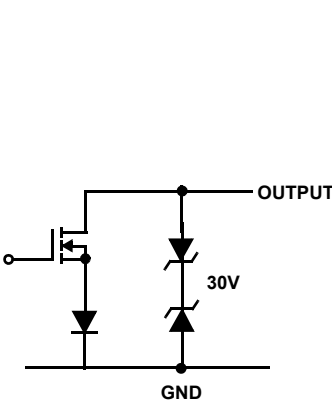
Figure 5. CANL Output
