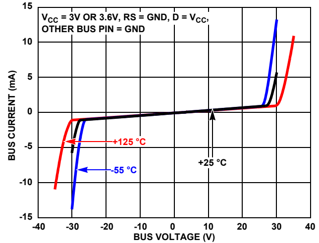
Figure 31. Bus Pin Leakage vs \pm 35V_{CM}
