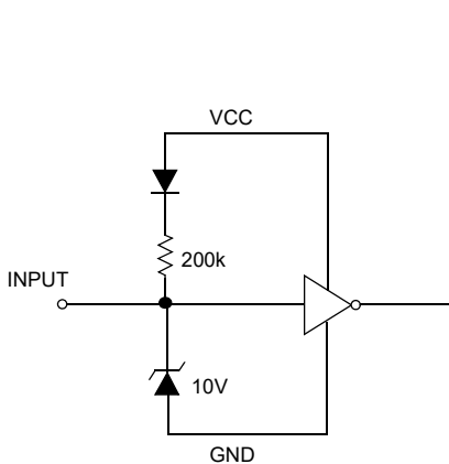
Figure 7. D Input
