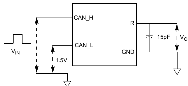
Figure 17. Receiver Test Circuit
