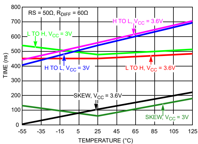
Figure 34. Transmitter Propagation Delay and Skew vs Temperature at Slow Speed
