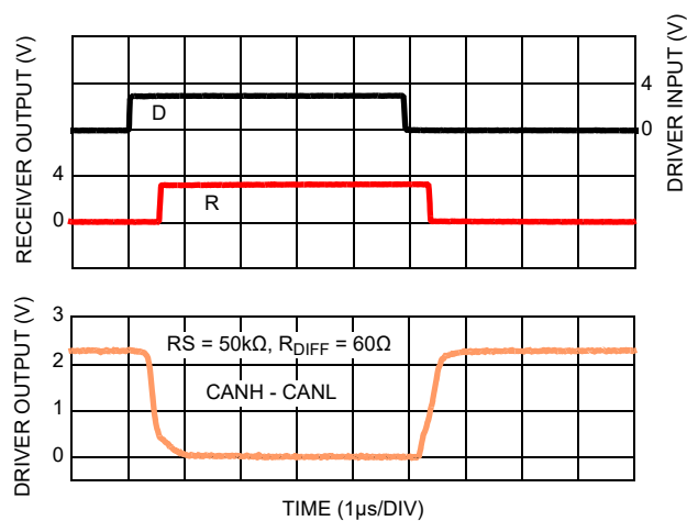
Figure 48. Slow Driver and Receiver Waveforms
