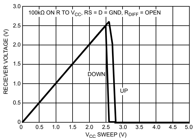
Figure 31. V_{CC} Undervoltage Lockout
