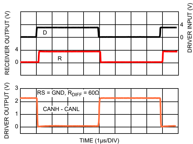
Figure 46. Fast Driver and Receiver Waveforms
