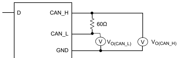
Figure 11. Driver Test Circuit
