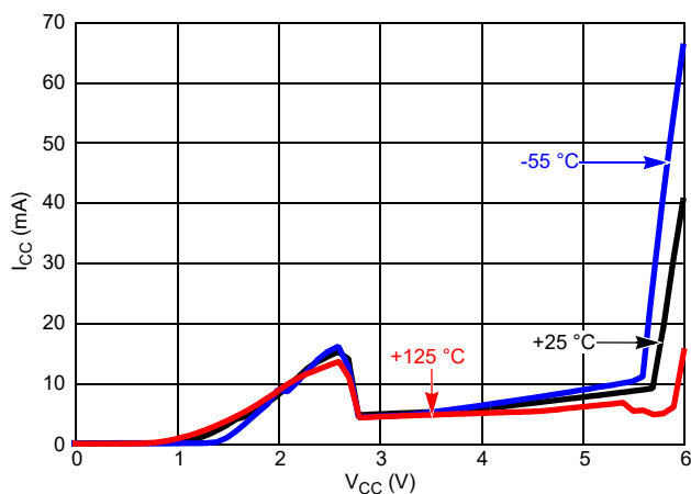
Figure 45. Supply Current vs Supply Voltage vs Temperature
