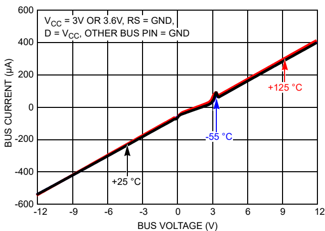
Figure 29. Bus Pin Leakage vs \pm 12V V_{CM}
