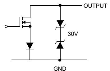
Figure 6. CANL Output
