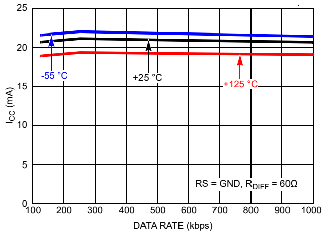
Figure 25. Supply Current vs Fast Data Rate vs Temperature
