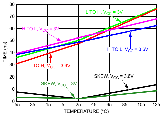
Figure 43. Receiver Propagation Delay and Skew vs Temperature
