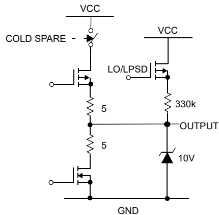
Figure 8. R Output
