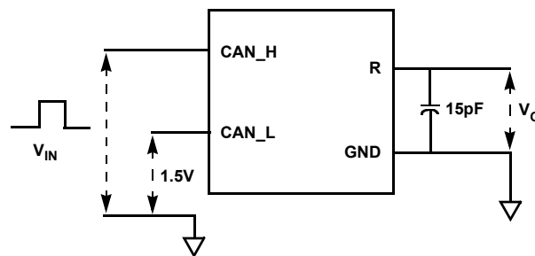
Figure 16. Receiver Test Circuit
