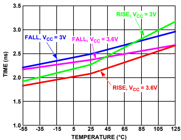
Figure 43. Receiver Rise and Fall Times vs Temperature
