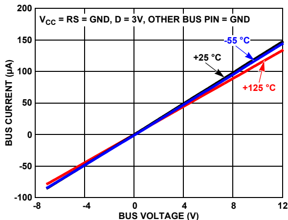
Figure 27. Bus Pin Leakage vs V_{CM} at V_{CC} = 0\text{V}
