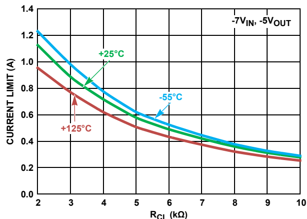
FIGURE 25. I_{CL} vs R_{CL} AND TEMPERATURE
