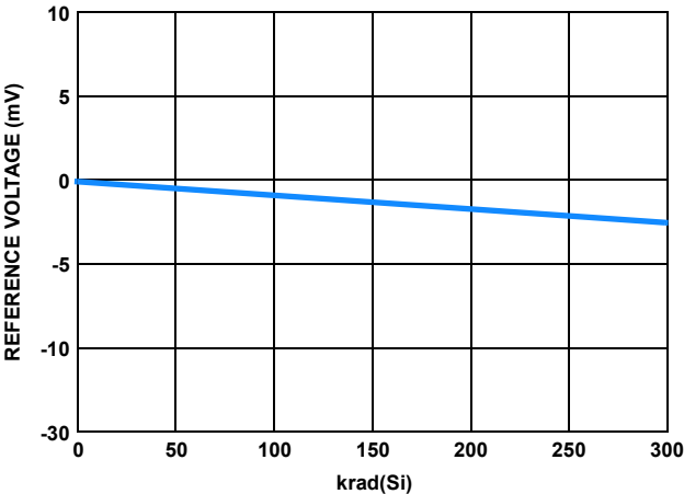
FIGURE 5. REFERENCE VOLTAGE CHANGE vs TOTAL DOSE RADIATION
