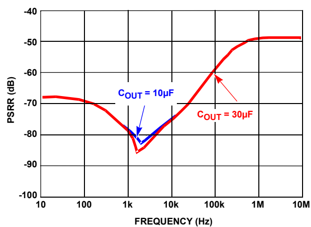
FIGURE 21. PSRR vs FREQUENCY ( V_{IN} = -7V , V_{OUT} = -5V )
