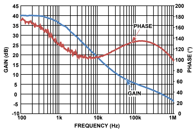
FIGURE 22. GAIN/PHASE -12V_{IN} , -5V_{OUT} , 0.5A I_{OUT}
