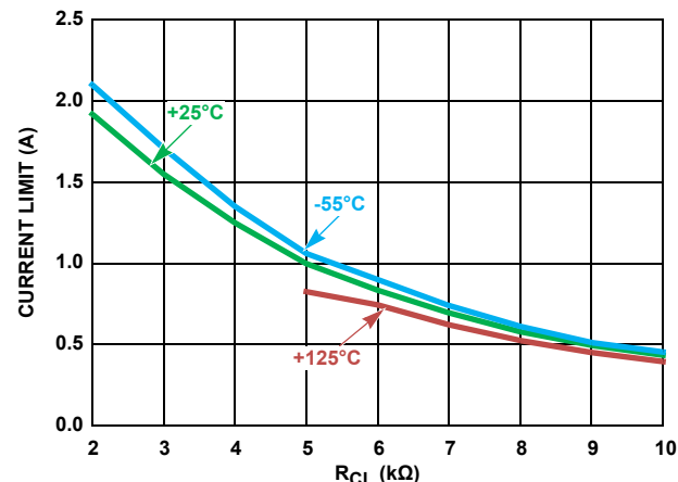
FIGURE 13. -20V_{IN} , -10V_{OUT}
