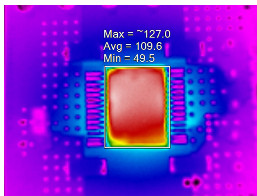
FIGURE 23. THERMAL ( V_{IN} = -12V , V_{OUT} = -5V , I_{OUT} = 0.74A , T_A = +25^{\circ}C )
