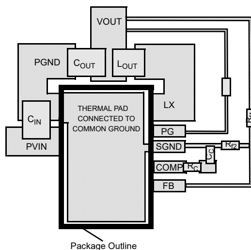
Figure 54. Layout Component Placement Suggestion
