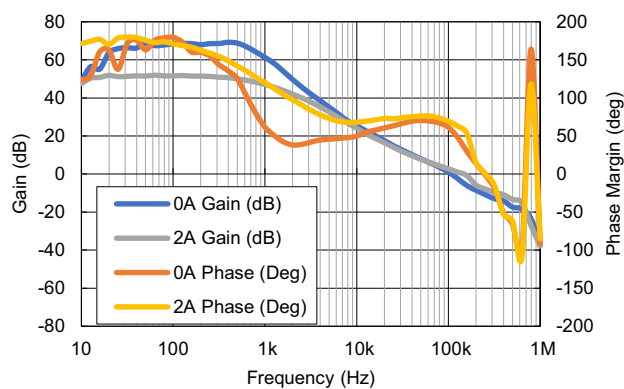
Figure 45. Ext Comp Gain/Phase BODE Plot, 3.3V IN , 1.0V OUT , 1MHz, R_{SLOPE} = 34.8k\Omega , R_{COMP} = 14k\Omega , C_{COMP} = 1200pF , L_{OUT} = 0.82\mu H , C_{OUT} = 172\mu F
