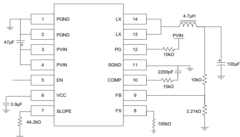
Figure 52. External Compensation Application Diagram for 12V to 3.3V, 500kHz
