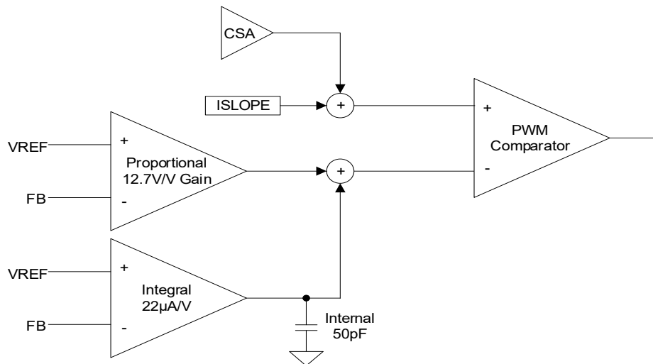
Figure 51. Internal Error Amplifier Block Diagram
