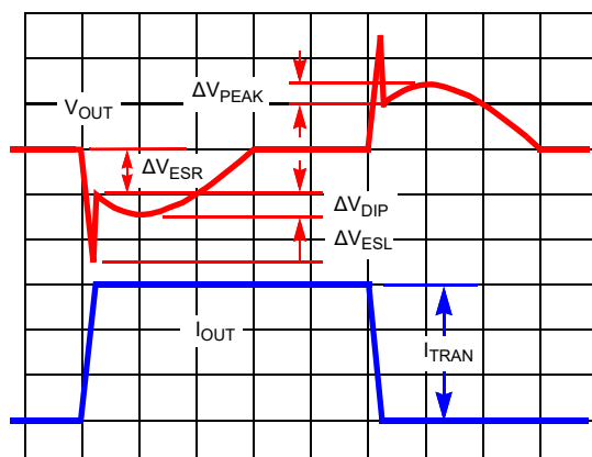
Figure 53. Typical Transient Response
