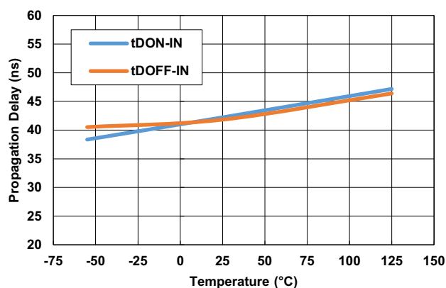
Figure 10. Input Propagation Delay vs Temperature
