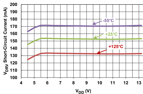
Figure 7. V_{DRV} Short-Circuit Current vs Temperature
