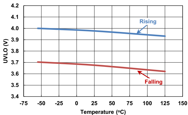
Figure 6. V_{DRV} Undervoltage Lockout Threshold
