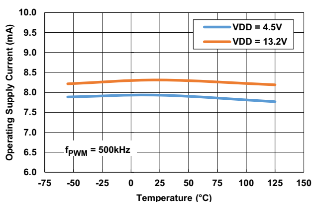
Figure 13. V_{DD} Operating Supply Current vs Temperature
