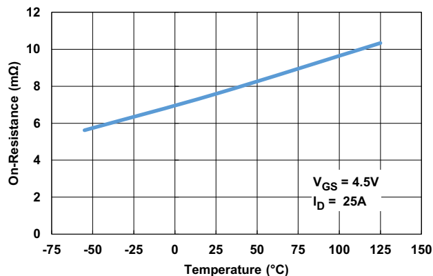
Figure 8. Drain-to-Source r_{DS(ON)} vs Temperature
