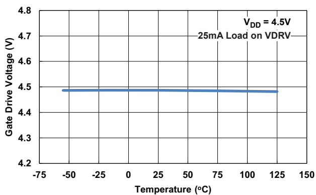
Figure 4. V_{DRV} vs Temperature
