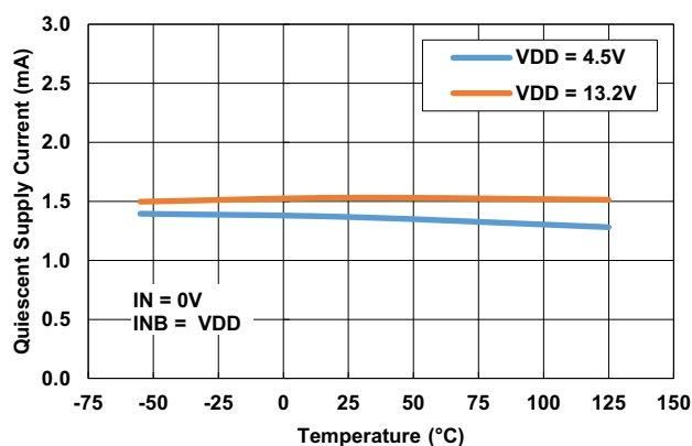
Figure 12. V_{DD} Quiescent Supply Current vs Temperature
