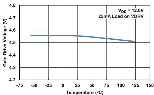
Figure 5. V_{DRV} vs Temperature
