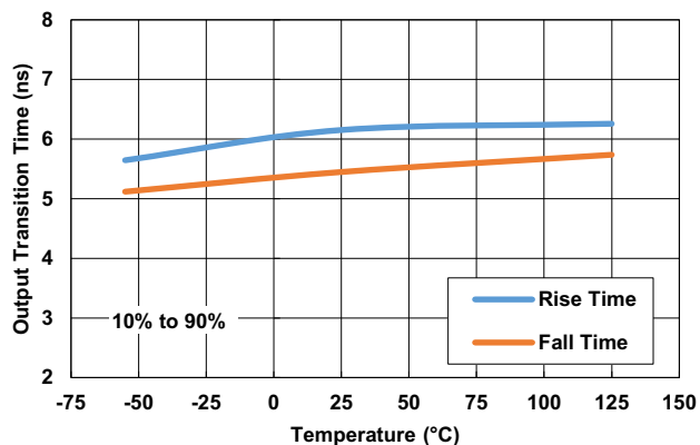
Figure 9. Output Transition Times vs Temperature
