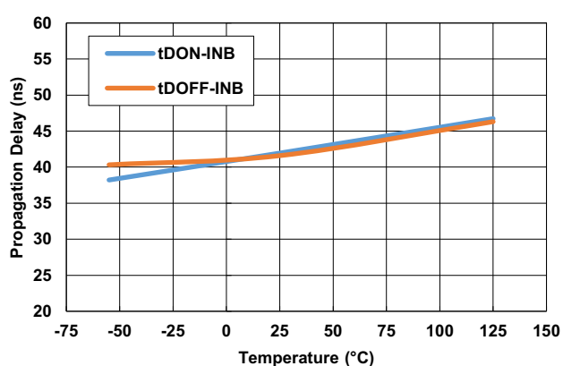
Figure 11. Input Bar Propagation Delay vs Temperature
