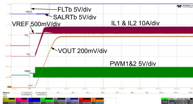
Figure 76. OPERATION Bit Startup ( V_{DD} = 5V , PV_{IN} = 5V , V_{OUT} = 1V , I_{LOAD} = 50A , OPERATION = 0x00h to 0x80h, SS_CONFIG = 32ms)
