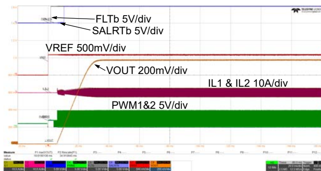
Figure 75. OPERATION Bit Startup ( V_{DD} = 5V , PV_{IN} = 5V , V_{OUT} = 1V , I_{LOAD} = 0A , OPERATION = 0x00h to 0x80h, SS_CONFIG = 32ms)
