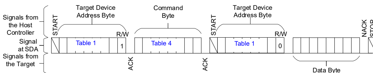
Figure 191. Read Byte
