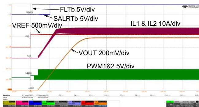
Figure 80. OPERATION Bit Startup ( V_{DD} = 5V , PV_{IN} = 5V , V_{OUT} = 1V , I_{LOAD} = 50A , OPERATION = 0x00h to 0x80h, SS_CONFIG = 64ms)
