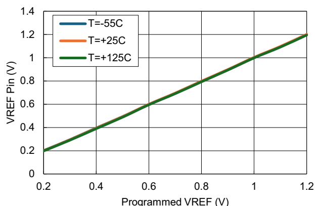
Figure 19. VREF Pin Voltage vs Programmed VREF value with V_{OUT\_COMMAND}
