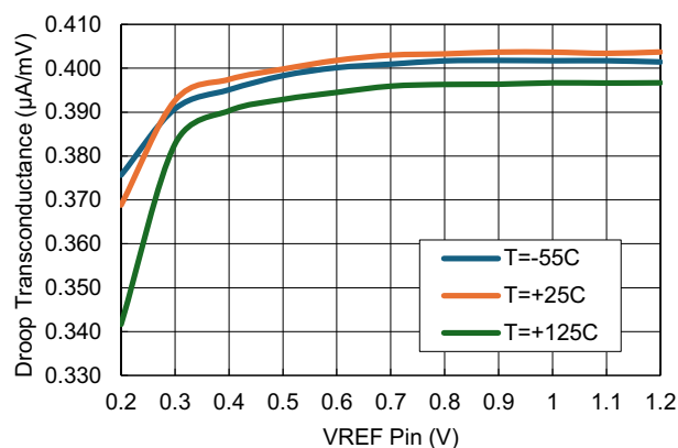
Figure 20. Droop Transconductance vs VREF Voltage
