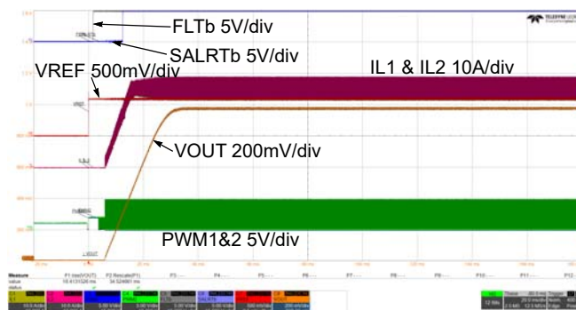
Figure 78. OPERATION Bit Startup ( V_{DD} = 19V , PV_{IN} = 12V , V_{OUT} = 1V , I_{LOAD} = 50A , OPERATION = 0x00h to 0x80h, SS_CONFIG = 32ms)
