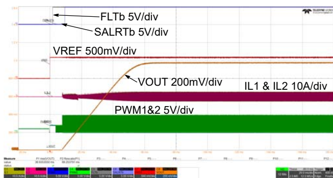
Figure 79. OPERATION Bit Startup ( V_{DD} = 5V , PV_{IN} = 5V , V_{OUT} = 1V , I_{LOAD} = 0A , OPERATION = 0x00h to 0x80h, SS_CONFIG = 64ms)
