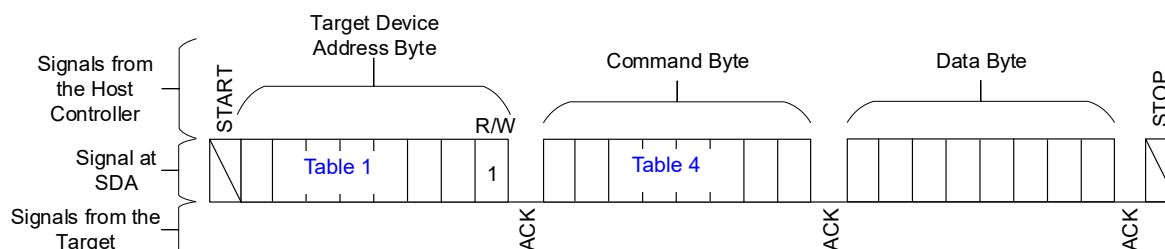
Figure 189. Write Byte
