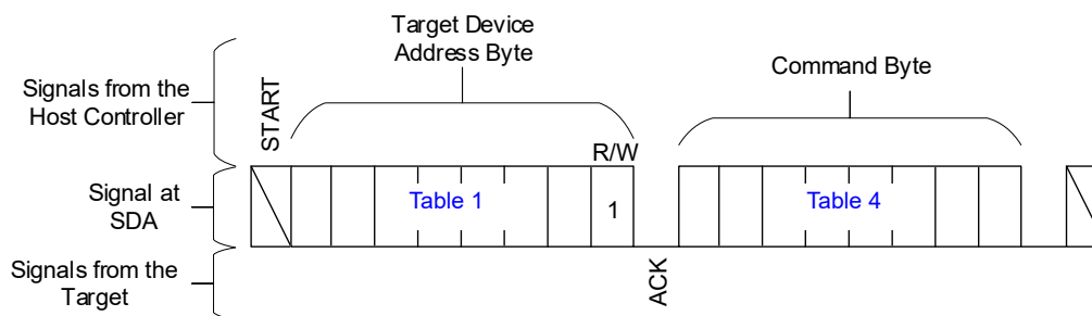
Figure 188. Send Byte
