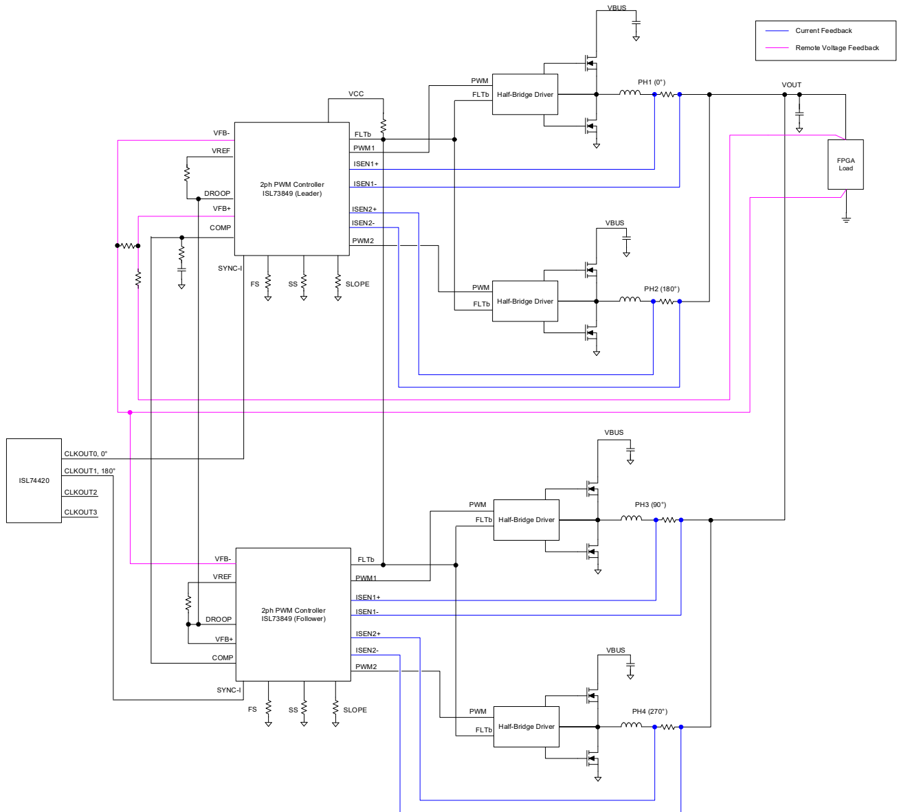
Figure 169. Leader-Follower Configuration for 4-Phase Operation
