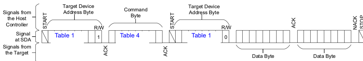
Figure 192. Read Word
