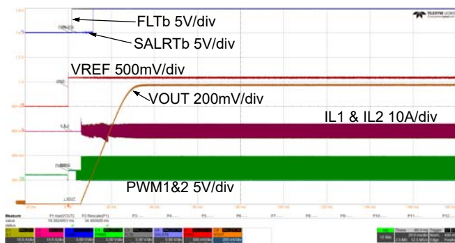
Figure 77. OPERATION Bit Startup ( V_{DD} = 19V , PV_{IN} = 12V , V_{OUT} = 1V , I_{LOAD} = 0A , OPERATION = 0x00h to 0x80h, SS_CONFIG = 32ms)
