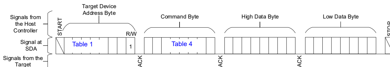
Figure 190. Write Word
