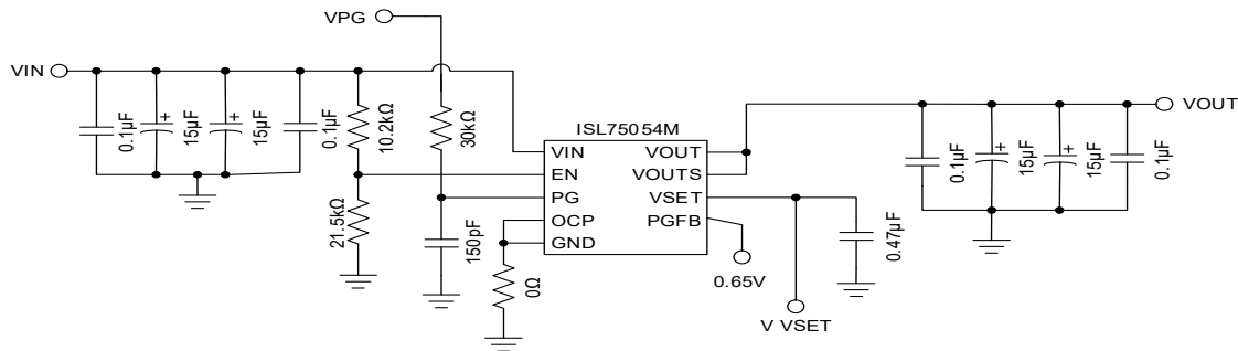
Figure 90. DSEE Test Schematic
