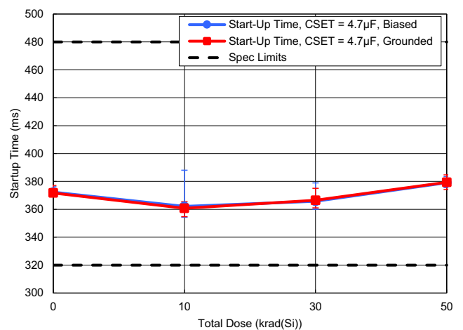
Figure 86. Startup Time with CSET = 4.7μF vs TID
