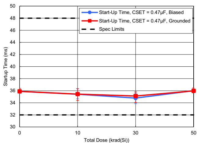
Figure 85. Startup Time with CSET = 0.47μF vs TID
