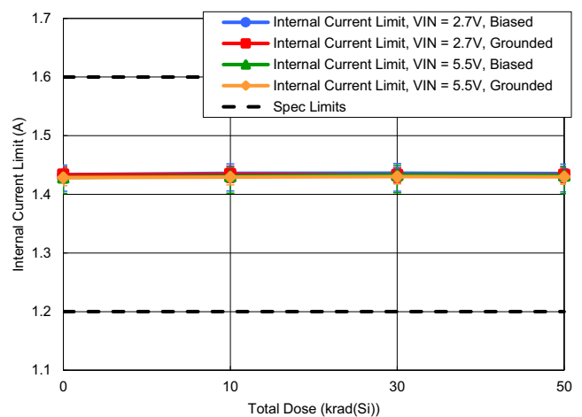
Figure 82. Internal Current Limit with V_{IN} = 2.7V or 5.5V vs TID
