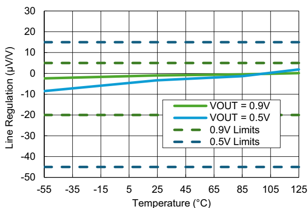
Figure 48. Line Regulation, \Delta V_{OS}/\Delta V_{IN}
