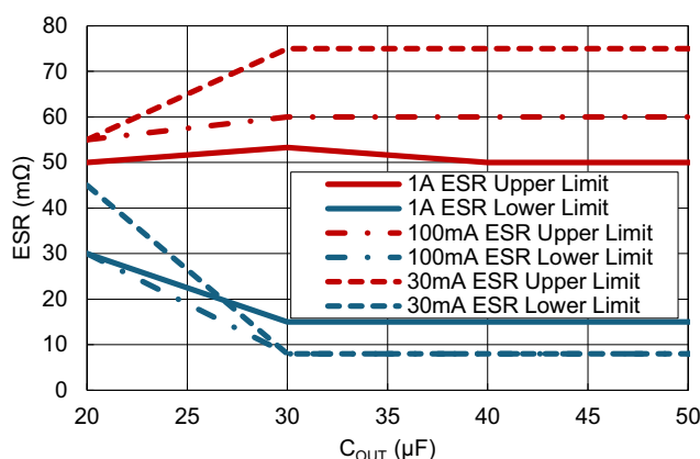
Figure 58. Recommended COUT and ESR Range for >60° Phase Margin
