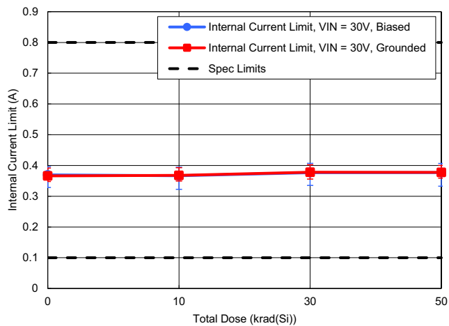
Figure 83. Internal Current Limit with V_{IN} = 30V vs TID
