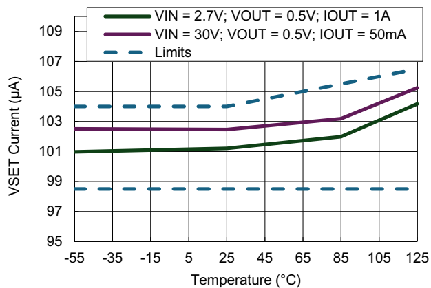
Figure 47. VSET Current, V_{OUT} = 0.5V
