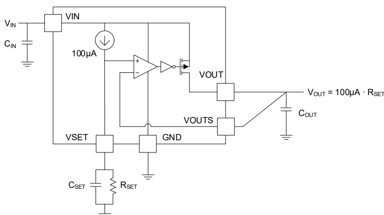
Figure 59. Functional Block for Output Regulation
