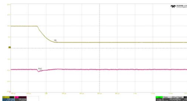
Figure 30. Line Transient ( V_{OUT} = 0.9V , V_{IN} = 12V to 2.7V , I_{OUT} = 1A , Slew Rate = 36.5V/ms )
