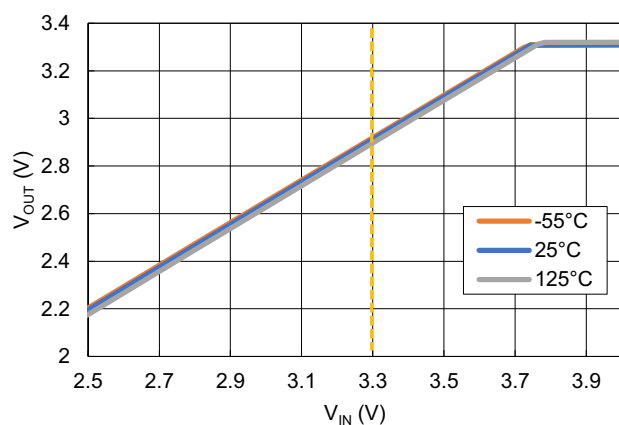
Figure 40. Dropout ( I_{OUT} = 1A , R_{SET} = 33.2k\Omega )
