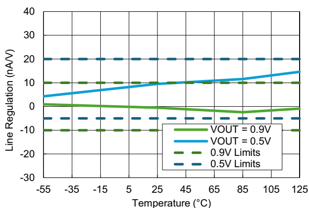
Figure 49. Line Regulation, \Delta I_{SET}/\Delta V_{IN}
