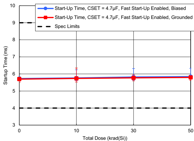
Figure 87. Startup Time with CSET = 4.7μF and Fast Startup Enabled vs TID
