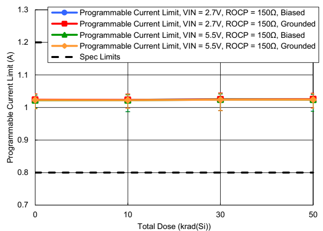
Figure 80. Programmable Current Limit with R_{OCP} = 150\Omega vs TID
