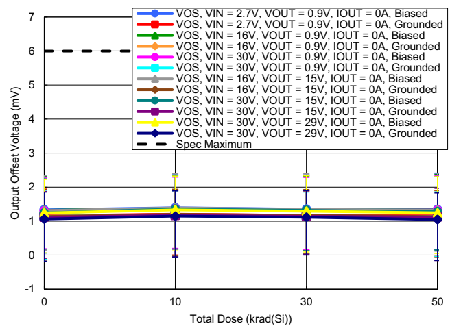
Figure 72. Output Offset Voltage with I_{OUT} = 0A vs TID
