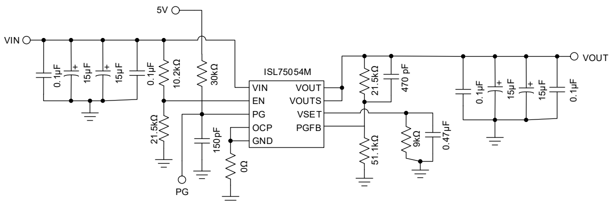
Figure 91. SET Test Schematic
