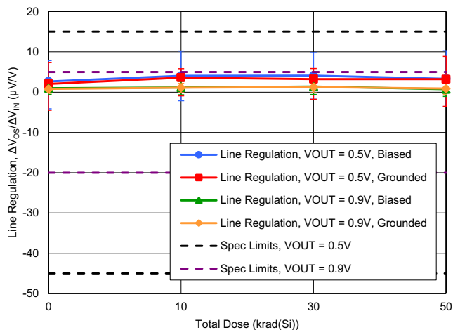
Figure 76. Line Regulation, \Delta V_{OS}/\Delta V_{IN} vs TID
