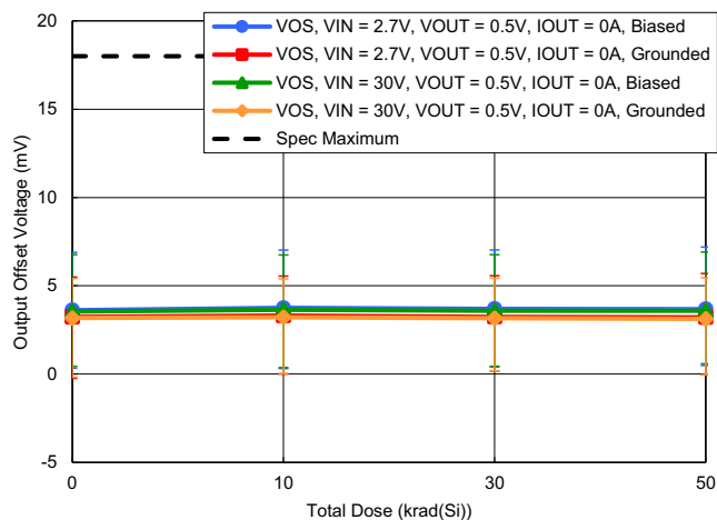
Figure 74. Output Offset Voltage with V_{OUT} = 0.5V and I_{OUT} = 0A vs TID
