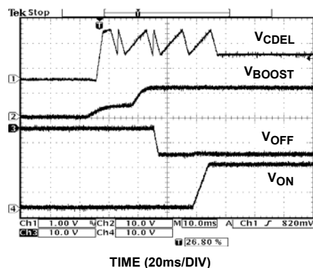
FIGURE 12. START-UP SEQUENCE
