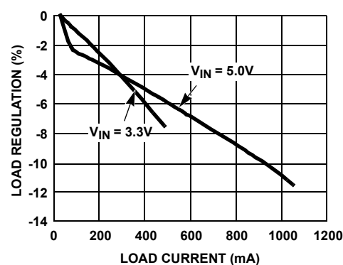
FIGURE 4. BOOST LOAD REGULATION vs LOAD CURRENT (P-MODE)
