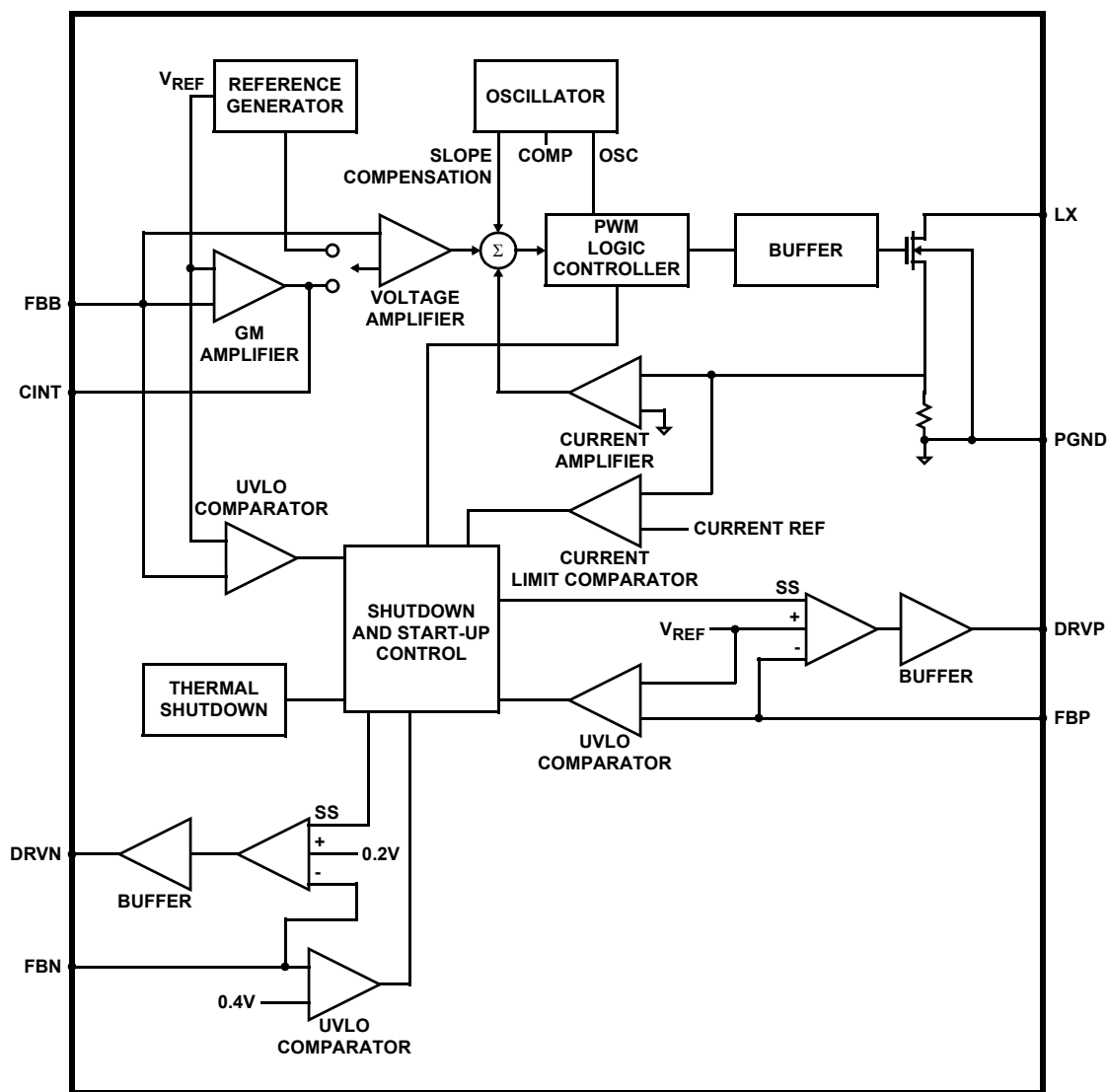
FIGURE 16. BLOCK DIAGRAM
