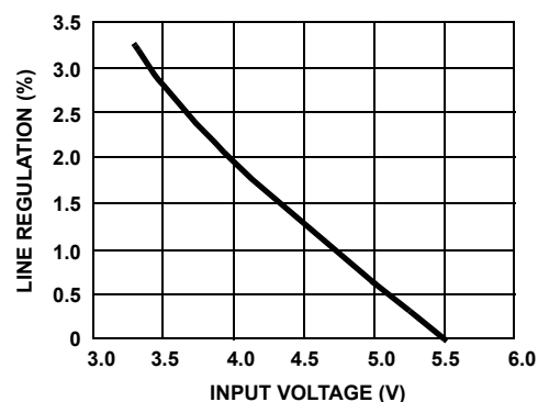
FIGURE 6. BOOST LINE REGULATION vs INPUT VOLTAGE (P-MODE)
