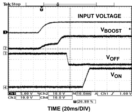
FIGURE 13. START-UP SEQUENCE
