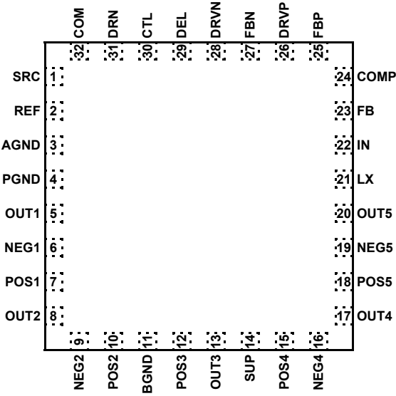
ISL78022 (32 LD TQFP) TOP VIEW
