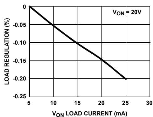
FIGURE 8. V_{\text{ON}} LOAD REGULATION
