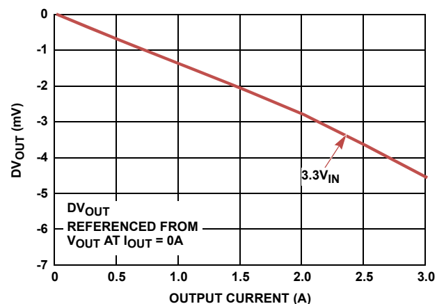
FIGURE 10. LOAD REGULATION, V_{OUT} = 1.8\text{V} , T_A = +25^\circ\text{C}
