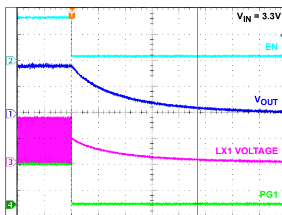
FIGURE 43. SOFT-DISCHARGE SHUTDOWN
