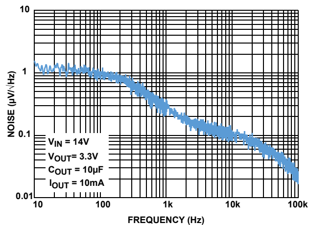
FIGURE 12. OUTPUT NOISE SPECTRAL DENSITY, I_{OUT} = 10mA
