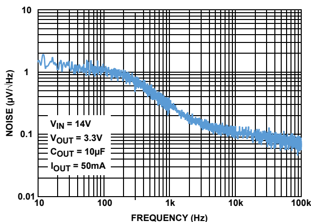
FIGURE 13. OUTPUT NOISE SPECTRAL DENSITY, I_{OUT} = 50mA
