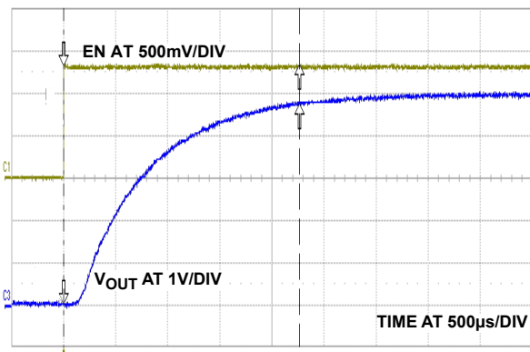
FIGURE 8. START-UP WAVEFORM
