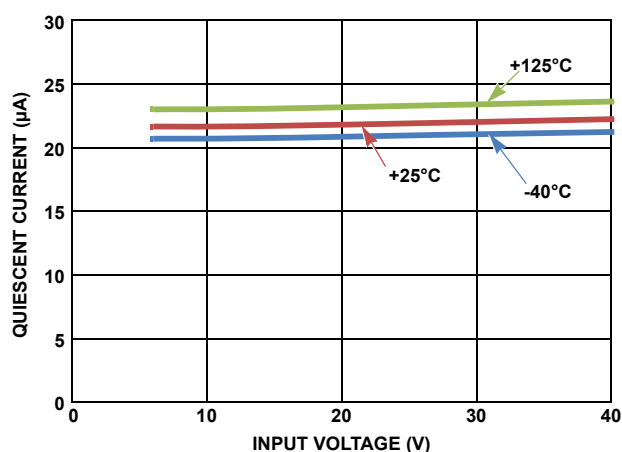
FIGURE 4. QUIESCENT CURRENT vs INPUT VOLTAGE (NO LOAD)
