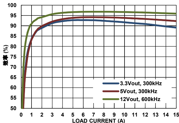
图 2。V IN = 24V
