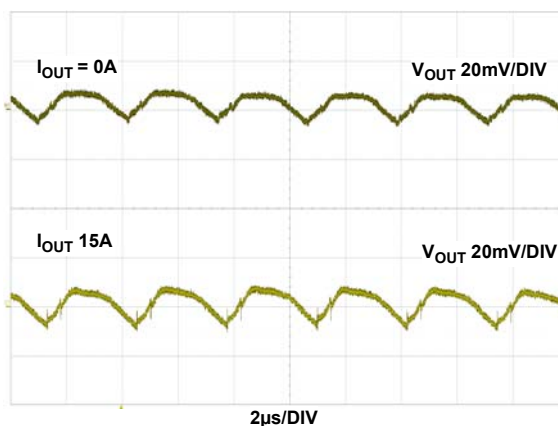
图 17。输出波纹, V_{OUT} = 3.3\text{V} , f_{SW} = 300\text{kHz} , C_{OUT} = 4 \times 100\mu\text{F} 陶瓷 + 1 \times 470\mu\text{F} POSCAP
