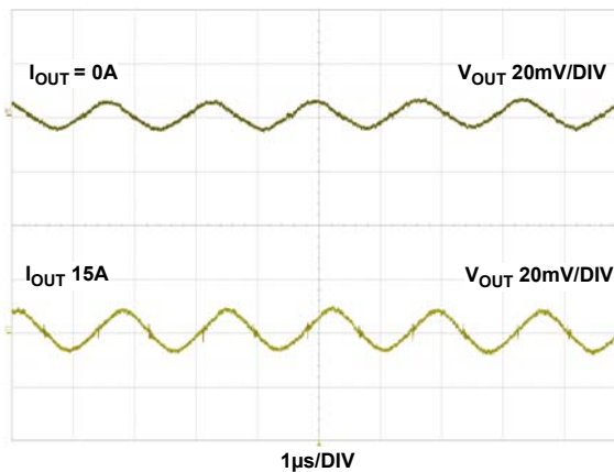
图 19。输出波纹, V_{OUT} = 12\text{V} , f_{SW} = 600\text{kHz} , C_{OUT} = 12 \times 22\mu\text{F} 陶瓷 + 2 \times 150\mu\text{F} POSCAP
