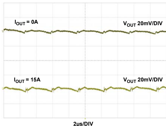
图 14。输出波纹, V_{OUT} = 1.2\text{V} , f_{SW} = 300\text{kHz} , C_{OUT} = 4 \times 100\mu\text{F} 陶瓷 + 1 \times 470\mu\text{F} POSCAP
