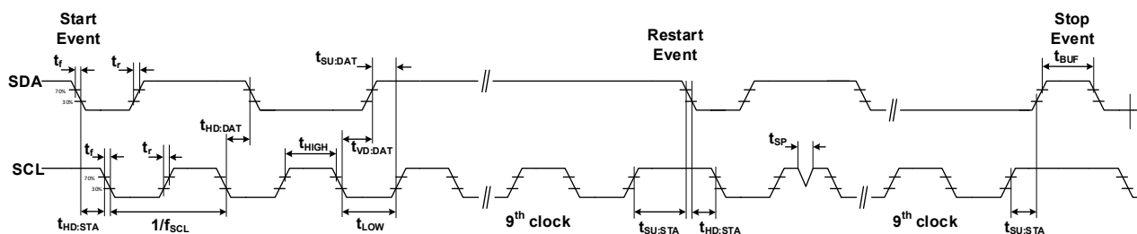
Figure 50. I 2 C Timing
