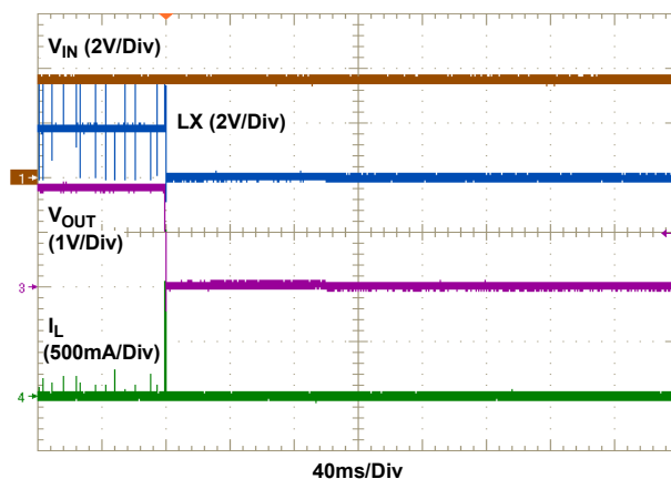
Figure 18. Output Short-Circuit Behavior (Shutdown Mode)
