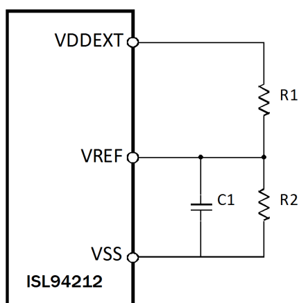
Figure 88. Cell Reading Accuracy Adjustment System
