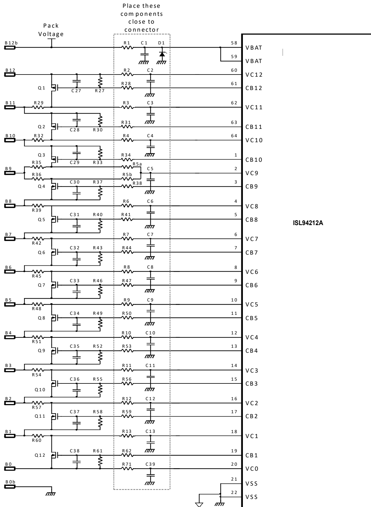
Figure 76. Battery Connection Circuits
