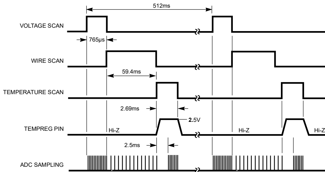
Figure 40. Scan Timing Example During Scan Continuous Mode and Scan All Mode
