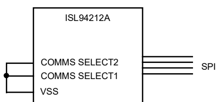
Figure 42. Non-Daisy Chain Communications Connections and Select
