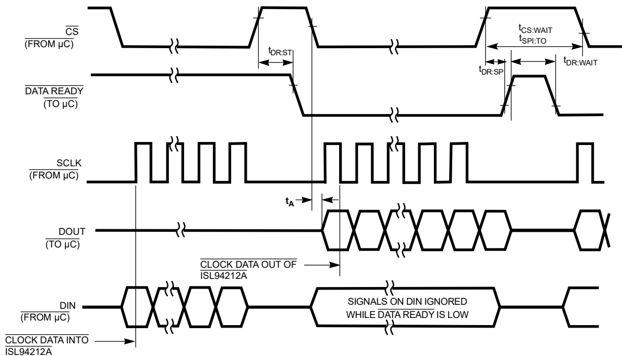
Figure 5. SPI Half Duplex (3-Wire) Interface Timing
