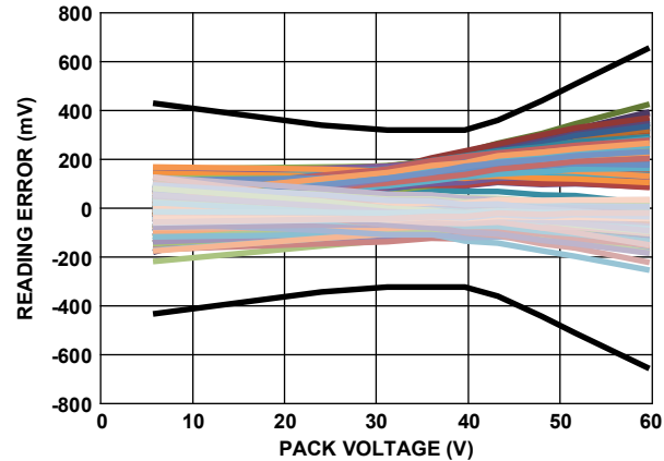
Figure 9. Pack Voltage Reading Error from -40°C to +85°C
