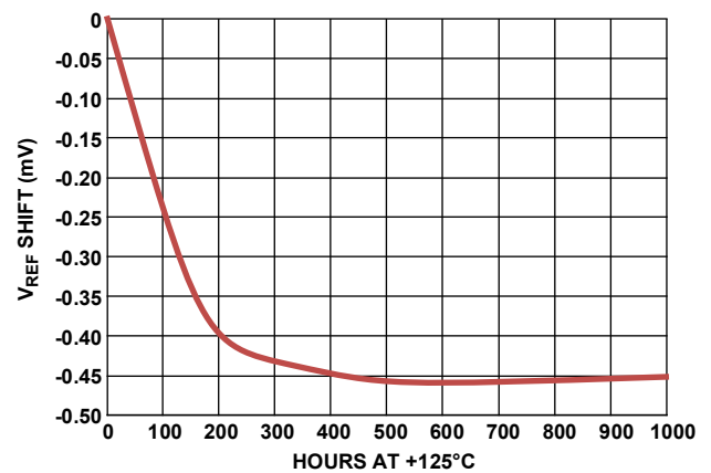
Figure 13. V_{REF} Shift Over HTOL
