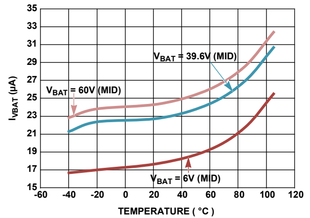
Figure 27. Pack Voltage Sleep Current vs Temperature at 6V, 39.6V, 60V (Daisy Chain Mode)
