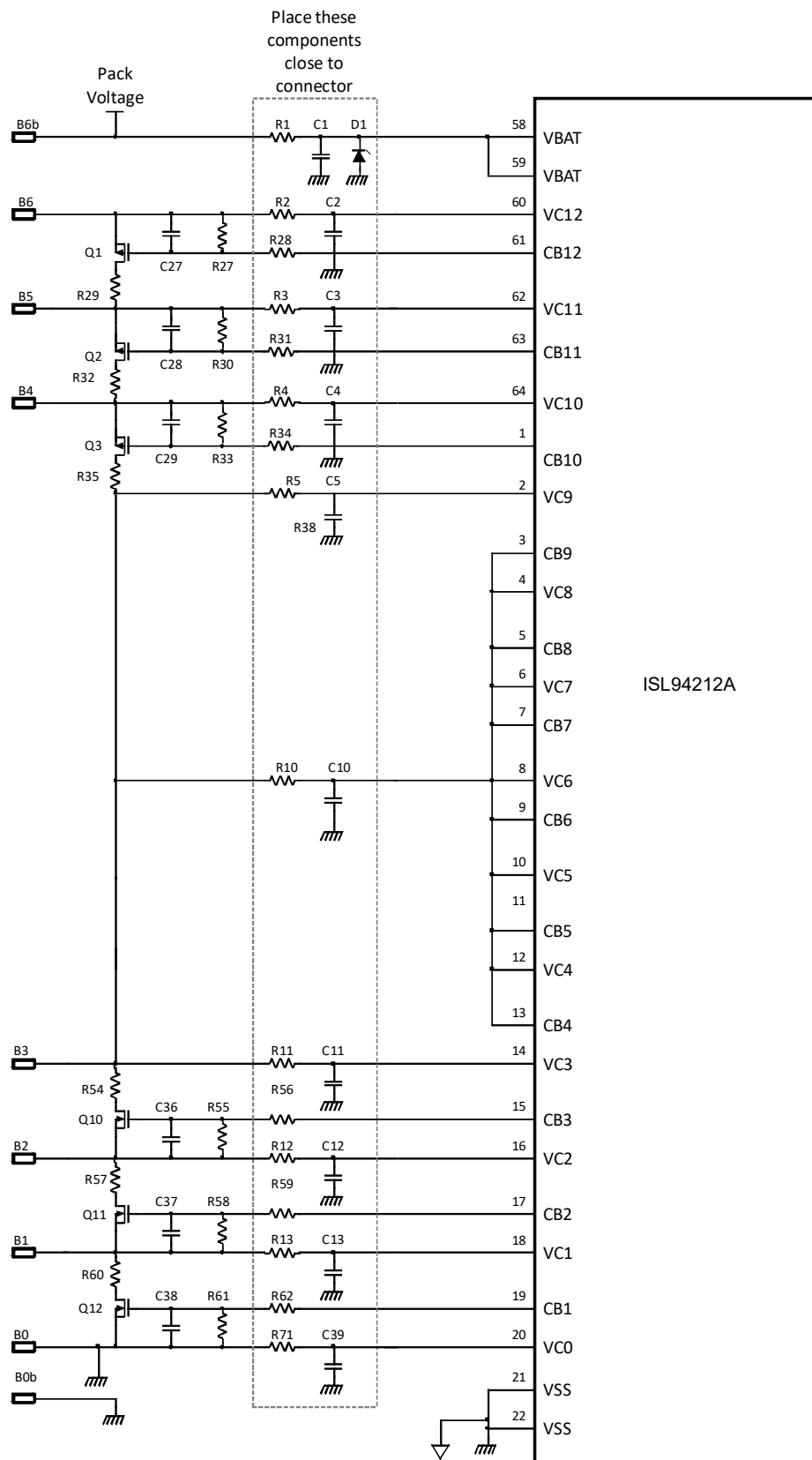
Figure 82. Battery Connection Circuits, System with 6 Cells
