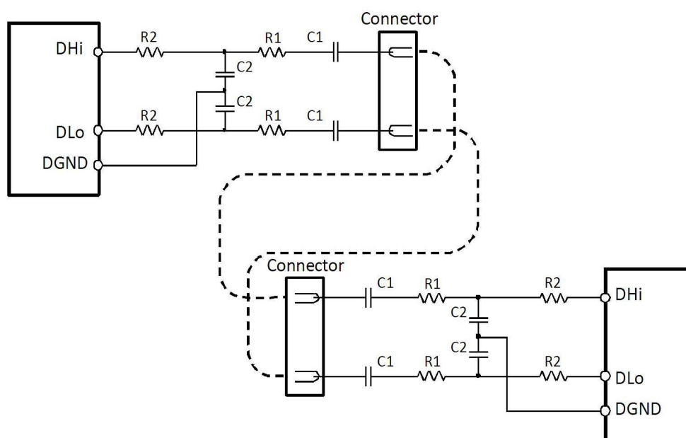
Figure 85. ISL94212A Daisy Chain Circuit Implementation
