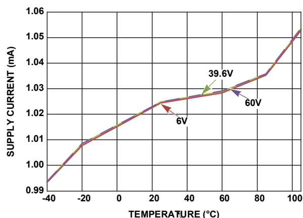
Figure 37. V3P3 Supply Current vs Temperature
