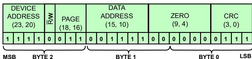
Figure 57. Device Level Command: Wake Up
