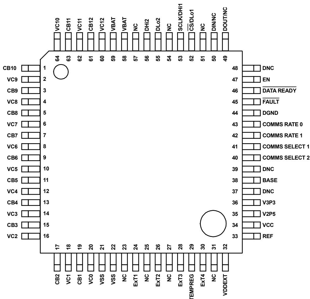
Figure 3. Pin Assignments – Top View
