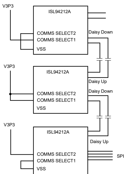
Figure 43. Daisy Chain Communications Connections and Selection
