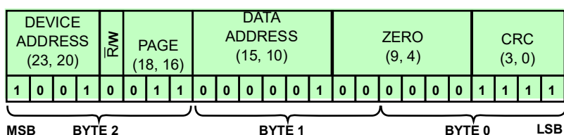
Figure 58. Device Level Command: Device 9, Scan Voltages
