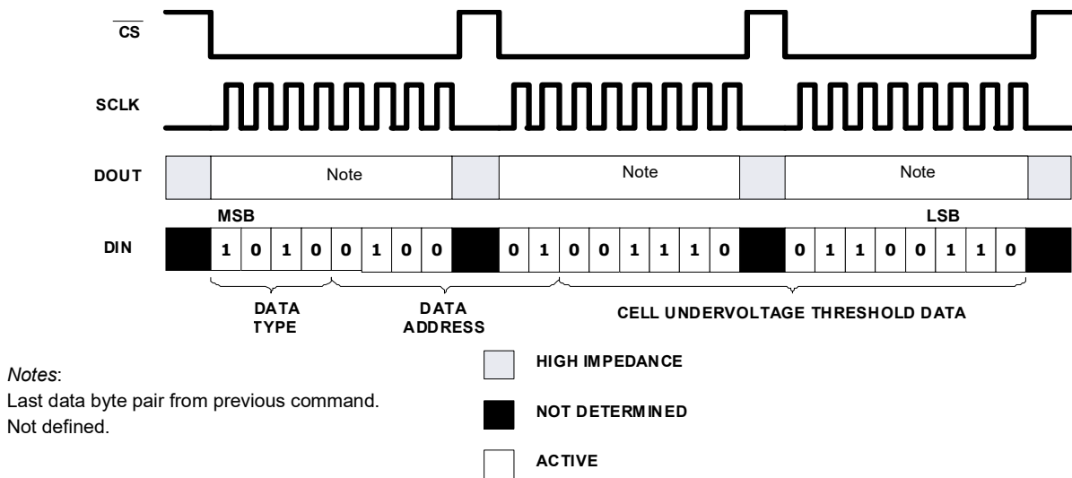
Figure 44. SPI Write Example: Write Undervoltage Threshold Data
