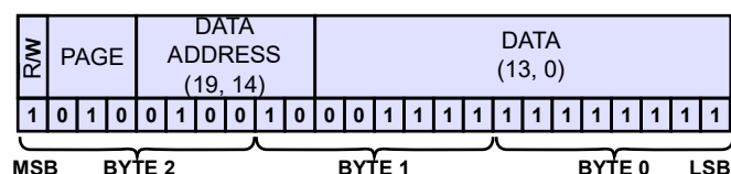
Figure 52. Device Write: Write External Temperature Limit = 14'h0FFF
