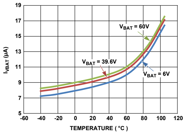
Figure 24. Pack Voltage Sleep Current vs Temperature at 6V, 39.6V, 60V (Standalone Mode)
