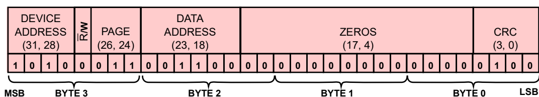
Figure 64. Device Communications Administration Response: Device 10, ACK
