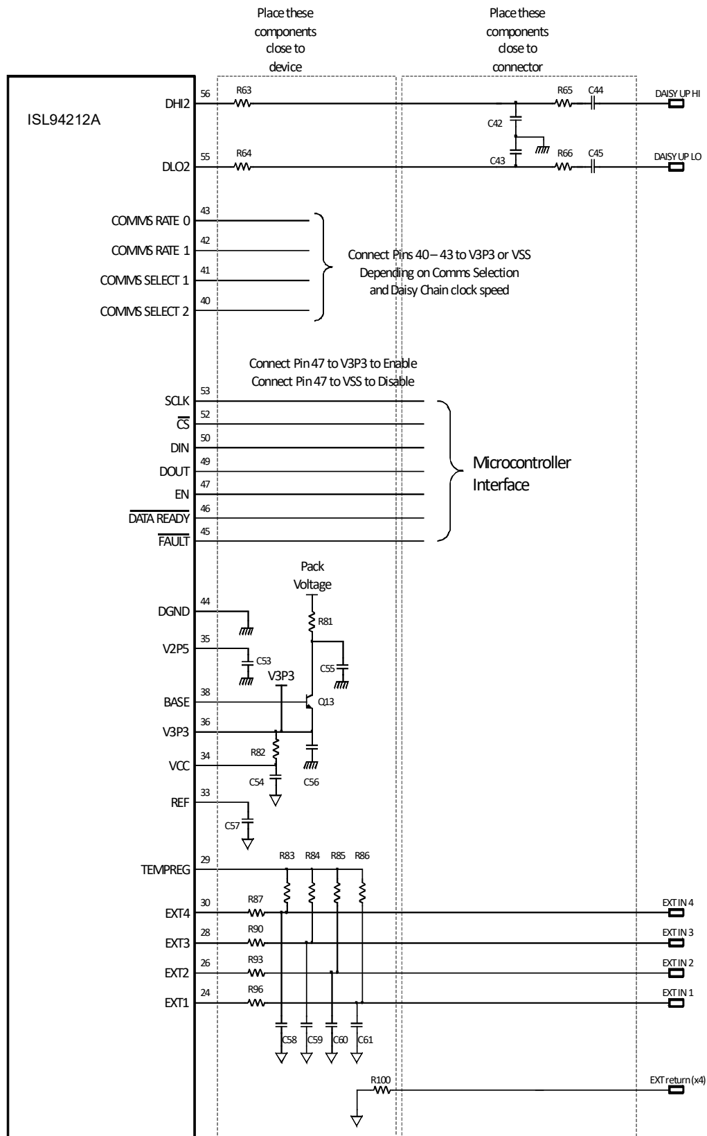
Figure 78. Non Battery Connections, Controller Daisy Chain Device
