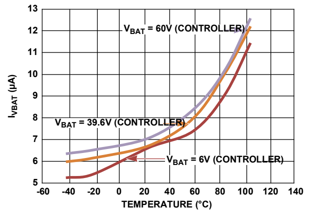
Figure 33. V_{BAT} Shutdown Current vs Temperature (EN = 0) at 6V, 39.6V, 60V
