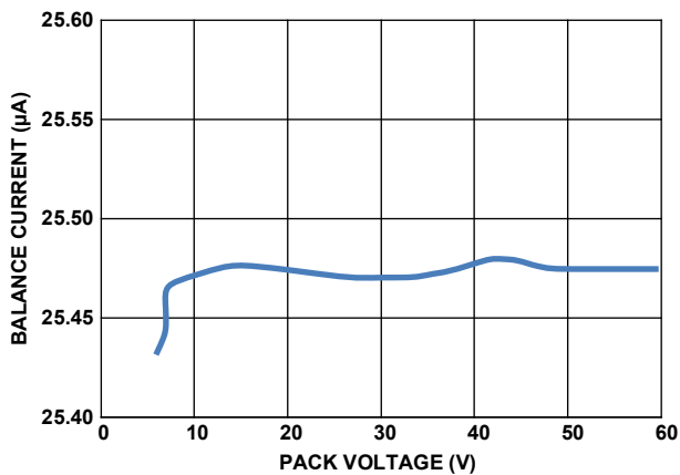
Figure 14. Balance Current vs Pack Voltage
