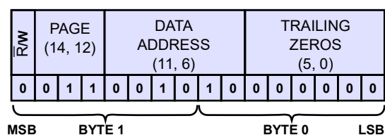
Figure 47. Device Level Command: Sleep
