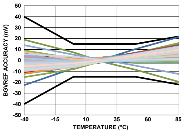
Figure 12. Voltage Reference Check Function vs Temperature ( V_{BAT} = 39.6 )
