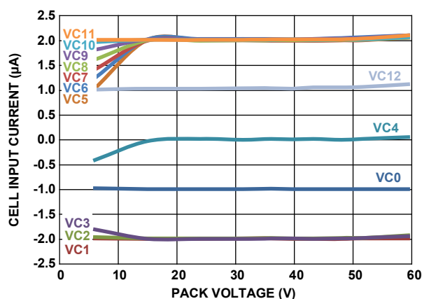
Figure 39. Cell Input Current vs Pack Voltage (+25°C)
