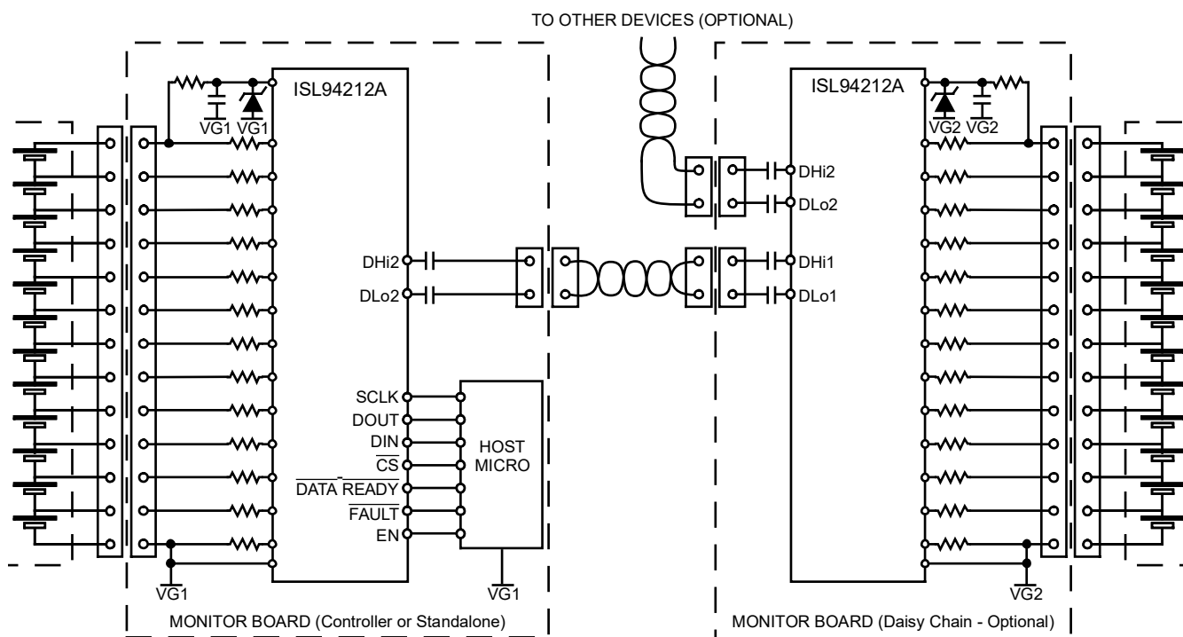
Figure 1. Typical Application Diagram
