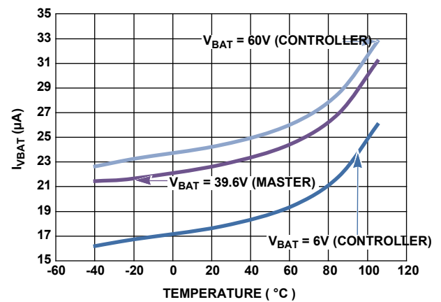
Figure 25. Pack Voltage Sleep Current vs Temperature at 6V, 39.6V, 60V (Daisy Chain Mode)
