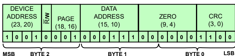
Figure 59. Device Read: Device 9, Get Cell 7 Data
