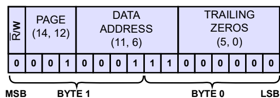
Figure 49. Device Read: Get Cell 7 Data
