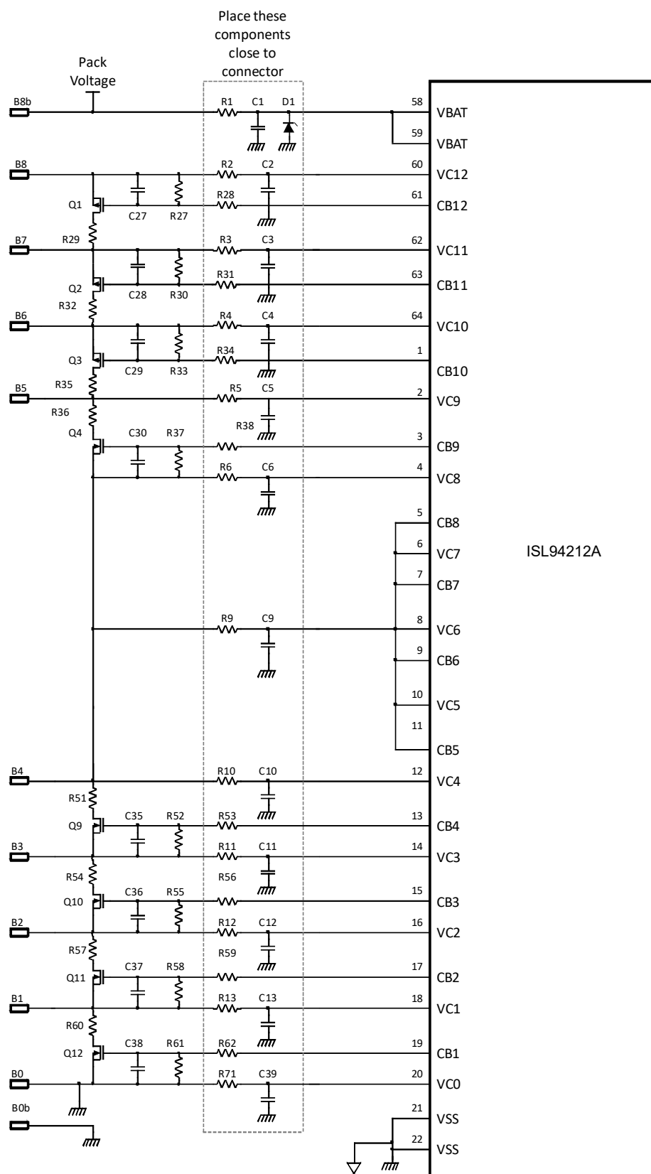
Figure 81. Battery Connection Circuits, System With 8 Cells
