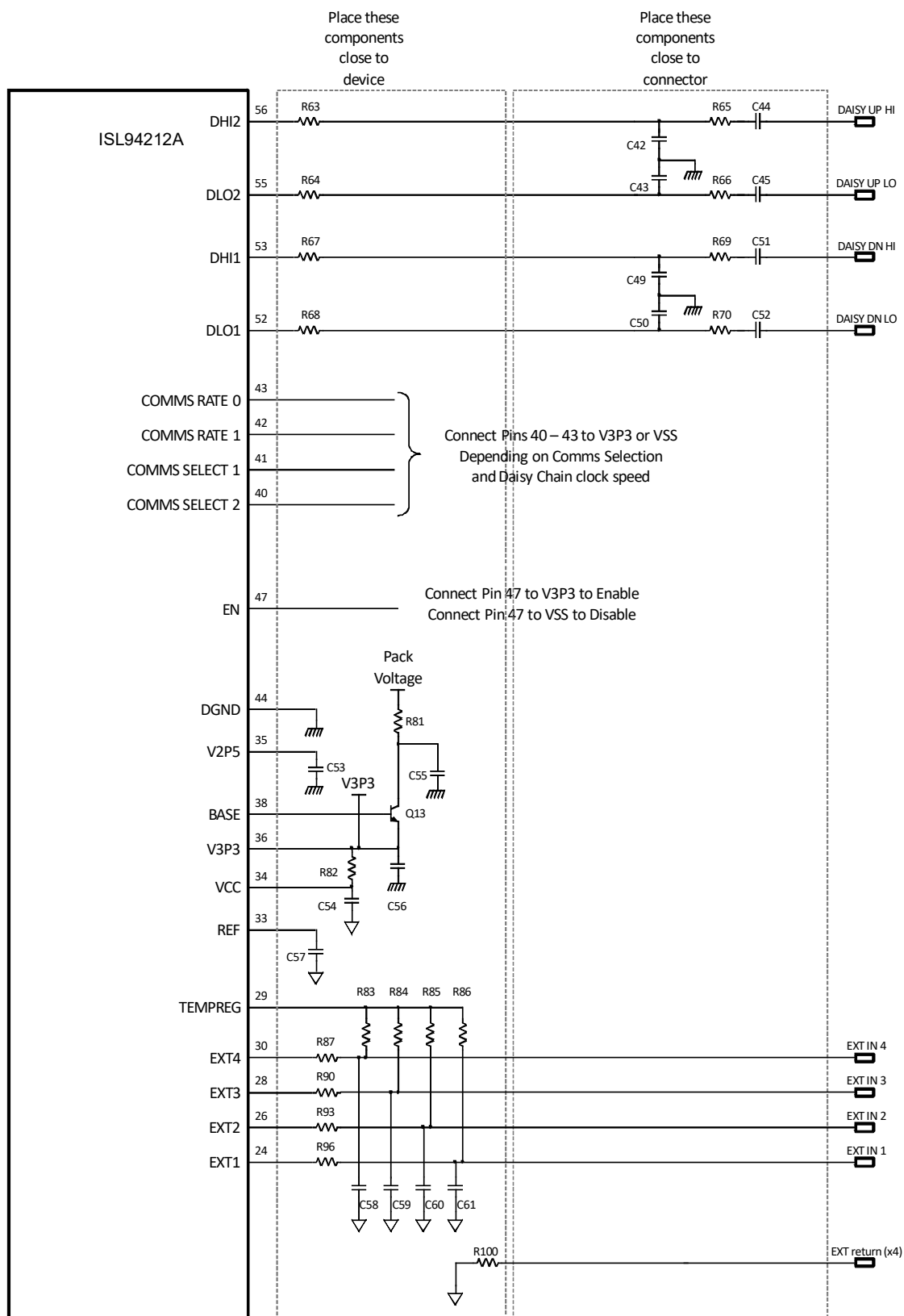
Figure 77. Non Battery Connections, Middle and Top Daisy Chain Devices
