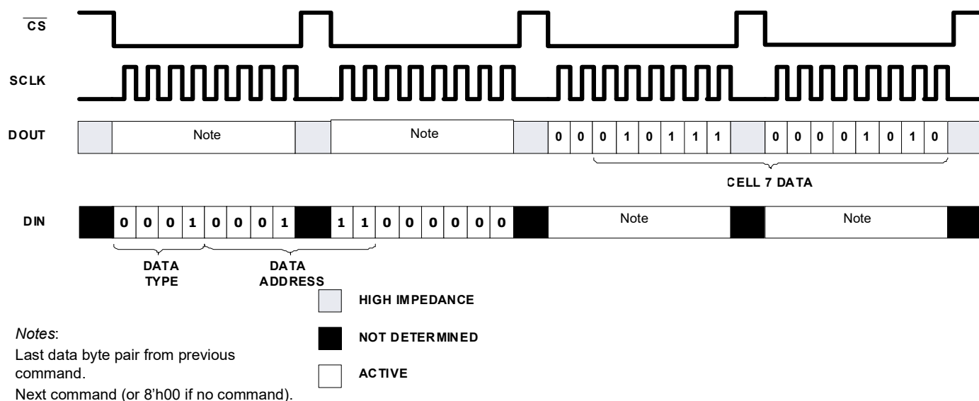
Figure 45. SPI READ EXAMPLE: READ CELL 7 DATA
