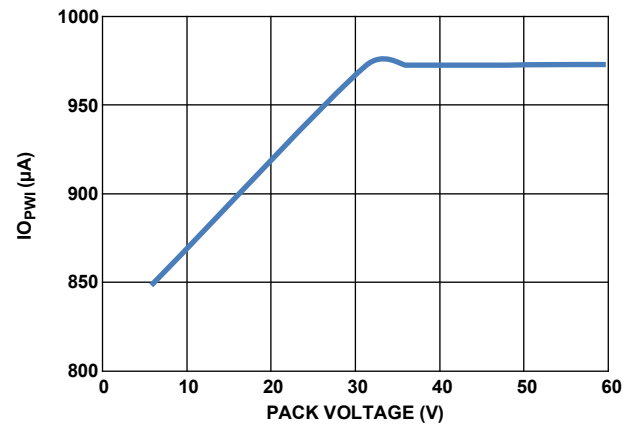
Figure 19. Open Wire Test Current vs Pack Voltage (1mA Setting)
