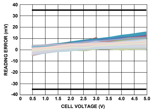
Figure 7. Cell Voltage Reading Error from -40°C to +85°C
