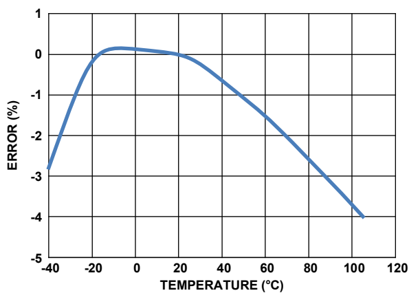
Figure 22. 32kHz Oscillator Error vs Temperature
