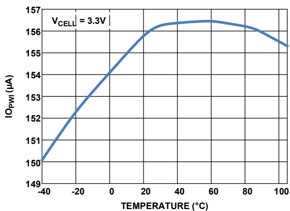
Figure 16. Open Wire Test Current vs Temperature (150 \mu A SETTING)
