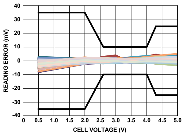
Figure 6. Cell Voltage Reading Error from 0°C to +50°C
