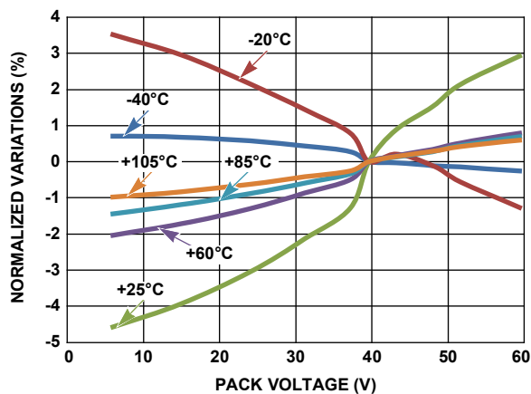
Figure 10. IC Temperature Error vs Pack Voltage
