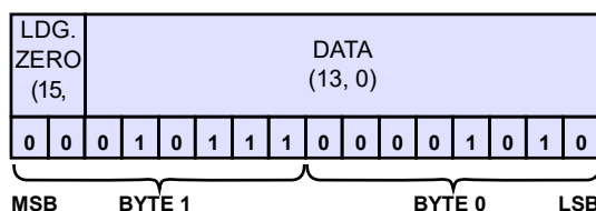
Figure 46. Non-Daisy Chain Device Response Example: Cell 7 Voltage = 16'h170A (3.6V)
