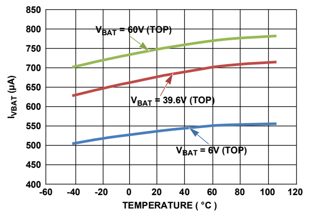
Figure 29. Pack Voltage Supply Current vs Temperature at 6V, 39.6V, 60V (Daisy Chain Top)
