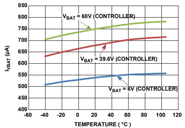
Figure 31. Pack Voltage Supply Current vs Temperature at 6V, 39.6V, 60V (Daisy Chain Controller)
