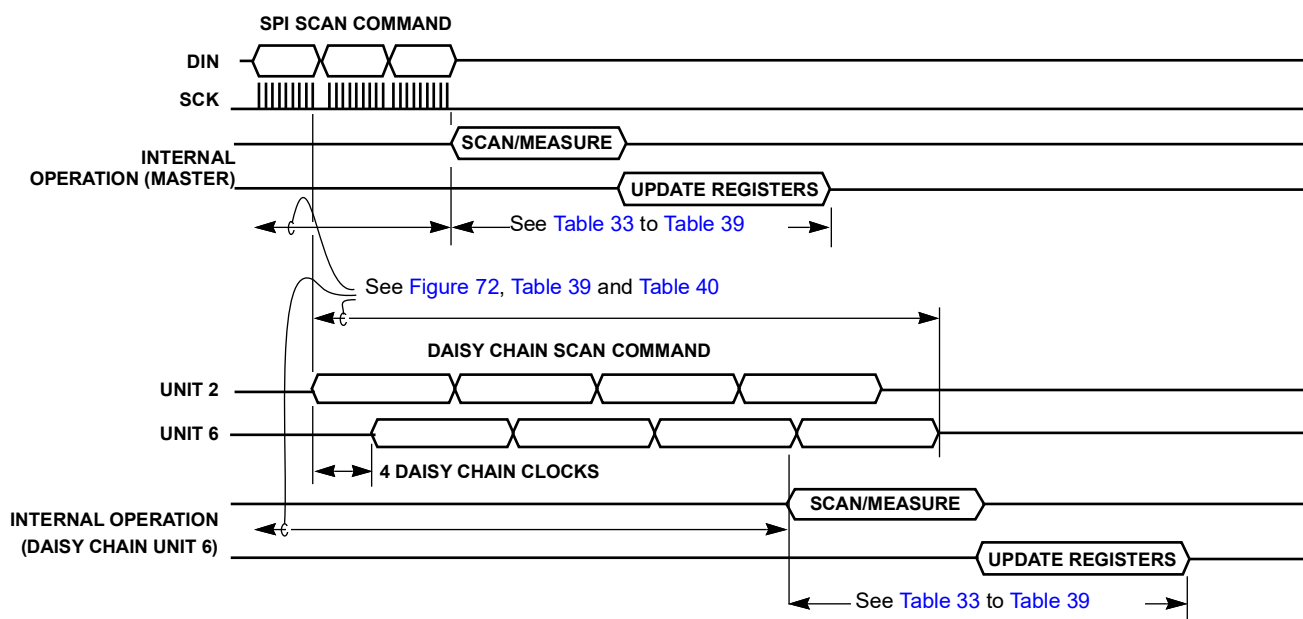
Figure 70. Measurement Timing (6 Device Daisy Chain)
