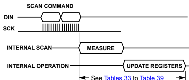
Figure 69. Measurement Timing (Standalone)
