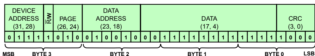
Figure 62. Device Write: Device 7, Write External Temperature Limit = 14'h0FFF
