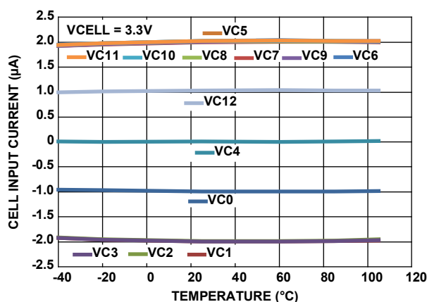
Figure 38. Cell Input Current vs Temperature
