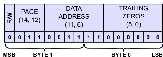
Figure 48. Device Level Command: Wake Up
