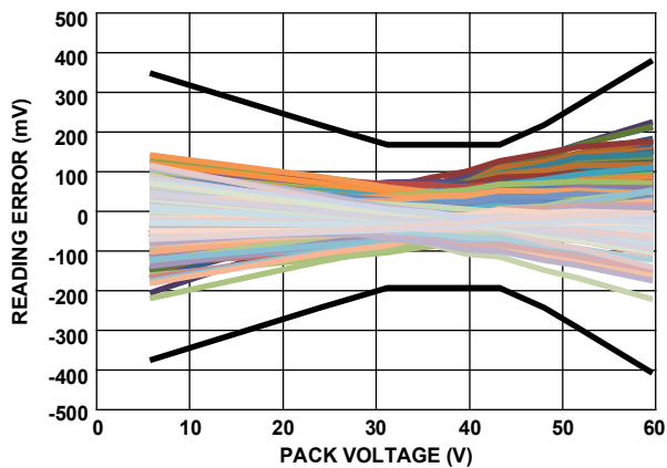
Figure 8. Pack Voltage Reading Error from 0°C to +50°C
