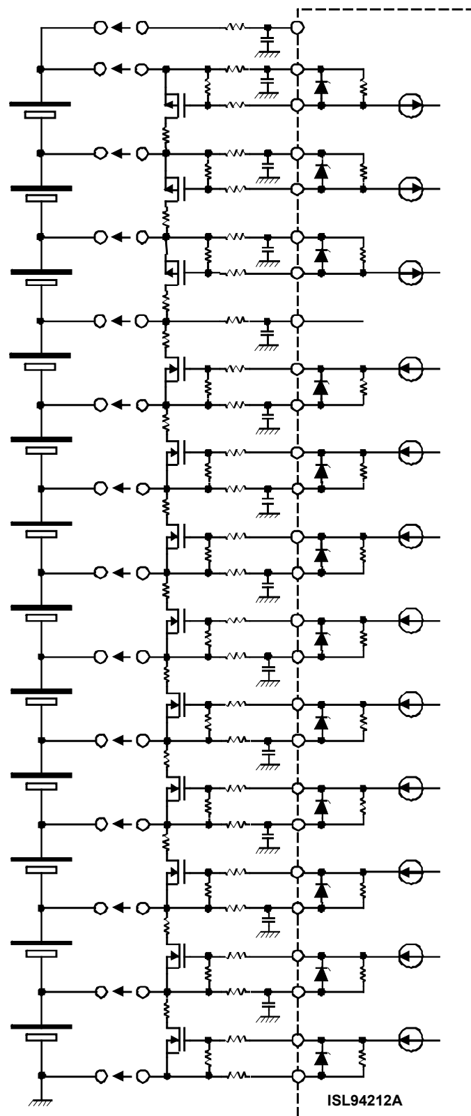
Figure 41. External Fet Driving Circuits
