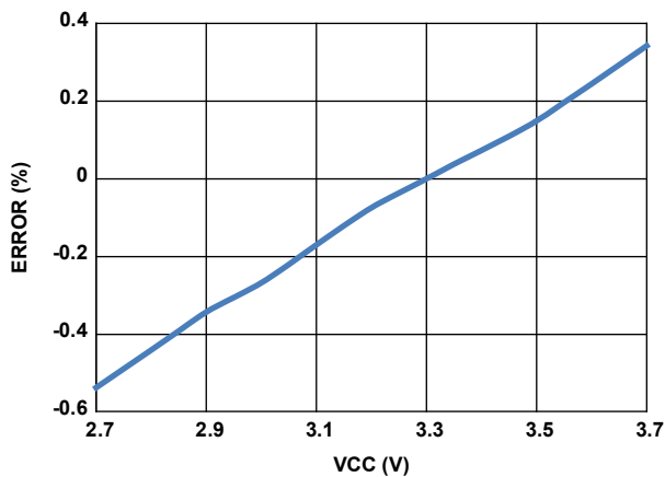
Figure 20. 4MHz Oscillator Error vs Vcc
