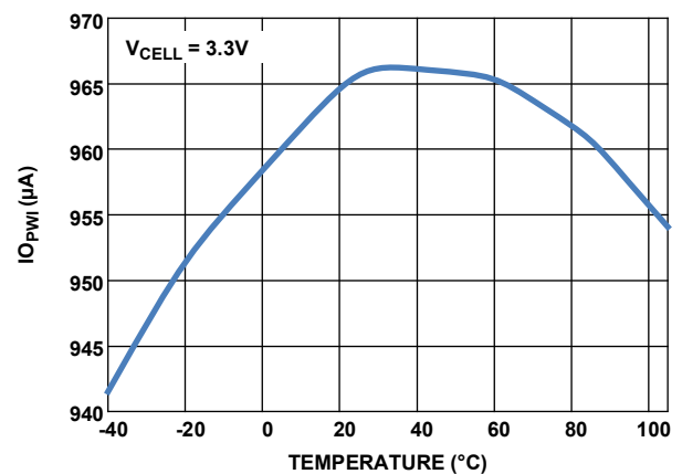
Figure 17. Open Wire Test Current vs Temperature (1mA Setting)
