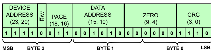
Figure 56. Device Level Command: Sleep
