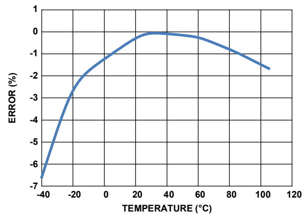
Figure 21. 4MHz Oscillator Error vs Temperature
