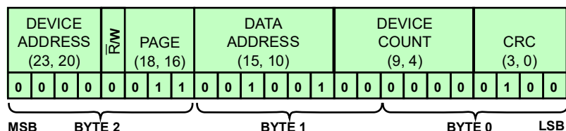
Figure 61. Identify Command
