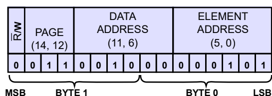
Figure 51. Device Level Command: Measure Cell 5 Voltage
