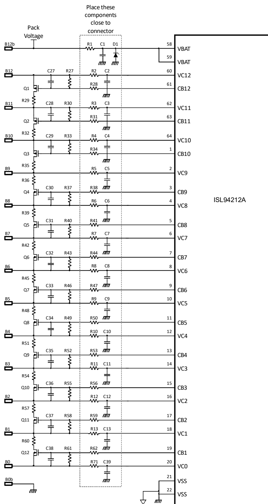
Figure 79. Battery Connection Circuits Alternative Configuration
