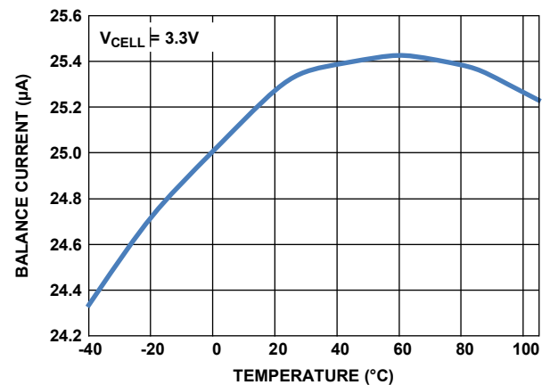
Figure 15. Balance Current vs Temperature
