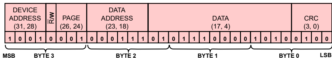
Figure 63. Device Data Response: Device 9, Cell 7 Voltage = 14'h170A (3.6V)
