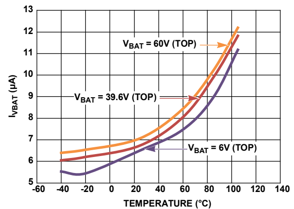
Figure 35. V_{BAT} Voltage Shutdown Current vs Temperature (EN = 0) AT 6V, 39.6V, 60V
