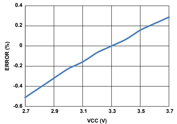
Figure 23. 32kHz Oscillator Error vs VCC
