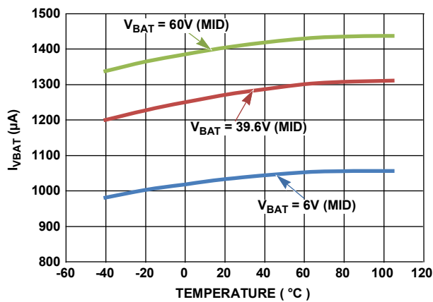
Figure 30. Pack Voltage Supply Current vs Temperature at 6V, 39.6V, 60V (Daisy Chain Middle)
