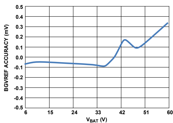
Figure 11. Voltage Reference Check Function vs Pack Voltage (at +25°C)
