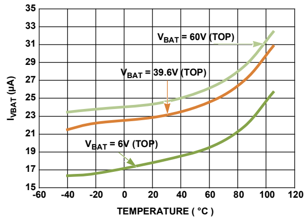
Figure 26. Pack Voltage Sleep Current vs Temperature at 6V, 39.6V, 60V (Daisy Chain Mode)
