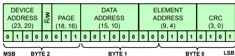
Figure 60. Element Level Command: Device 4, Measure Cell 5 Voltage
