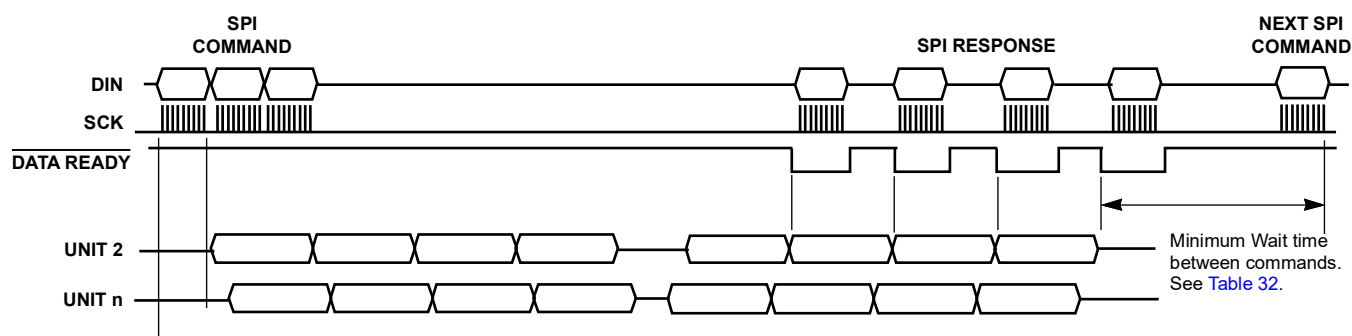
Figure 75. Minimum Wait Between Commands (Daisy Chain Response - Top Device)
