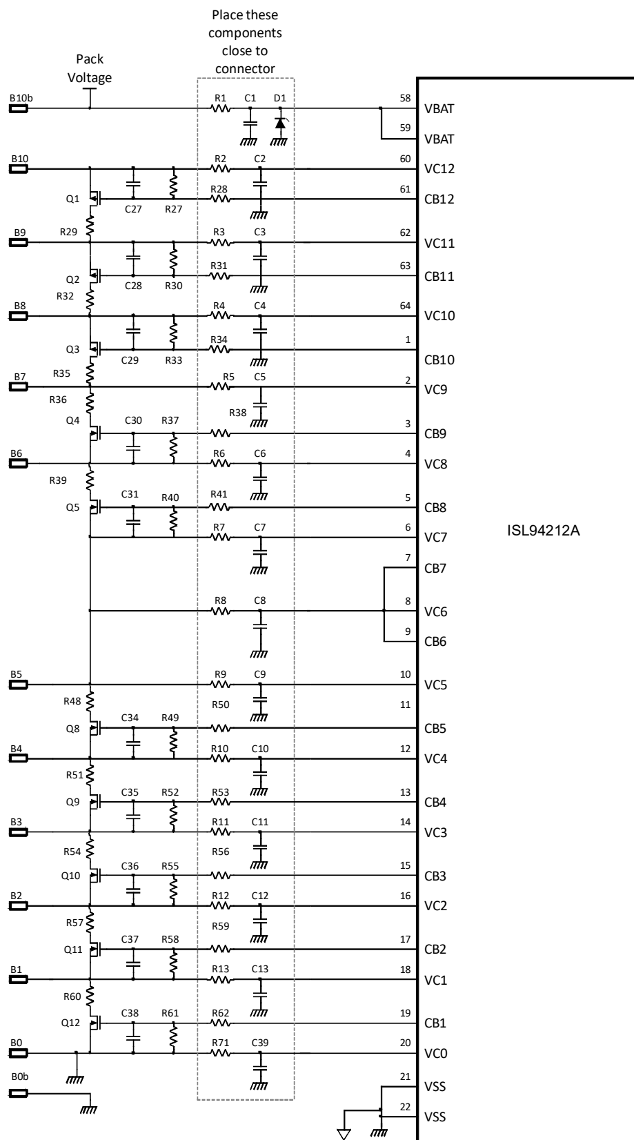
Figure 80. Battery Connection Circuits, System with 10 Cells
