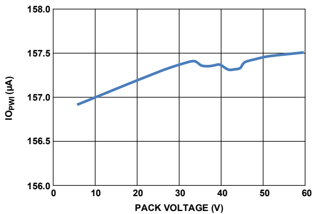
Figure 18. Open Wire Test Current vs Pack Voltage (150µA Setting)
