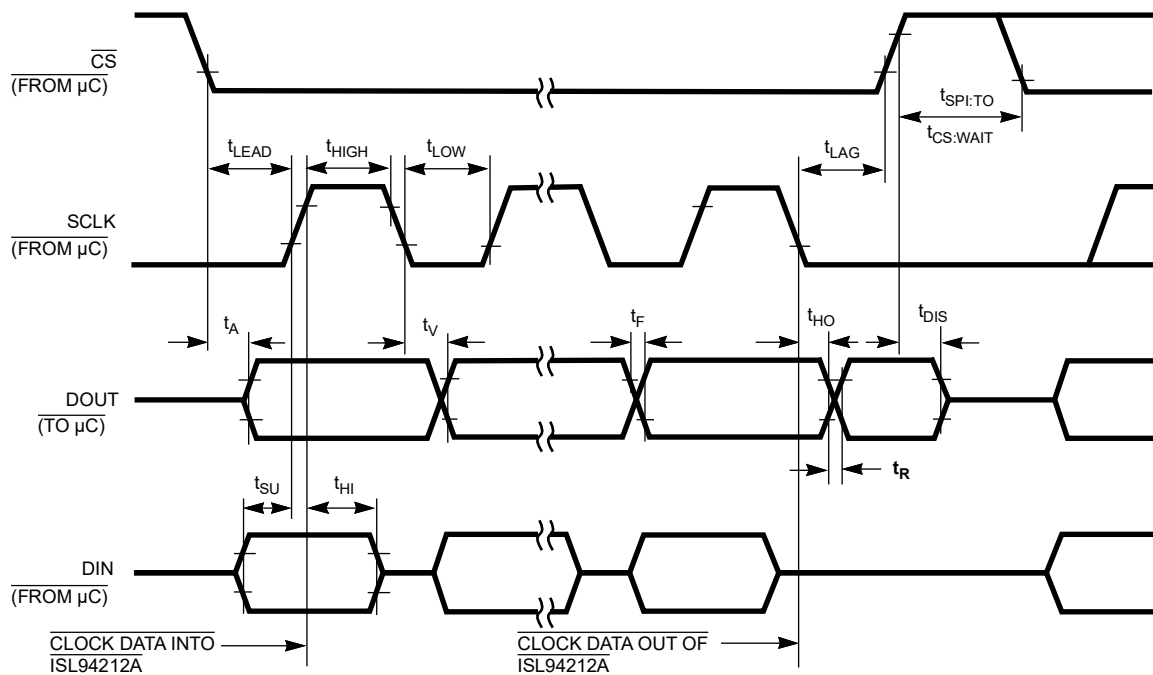
Figure 4. SPI Full Duplex (4-Wire) Interface Timing
