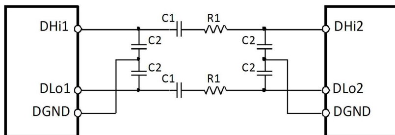
Figure 86. ISL94212A Daisy Chain – Board Level Implementation Circuit
