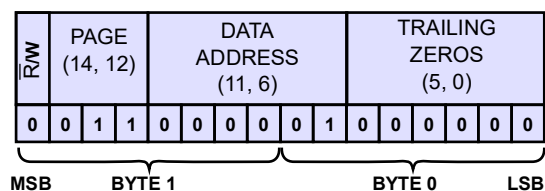
Figure 50. Device Level Command: Scan Voltages
