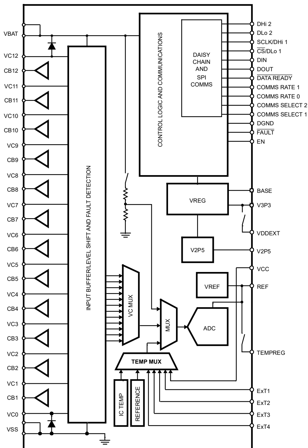
Figure 2. Block Diagram
