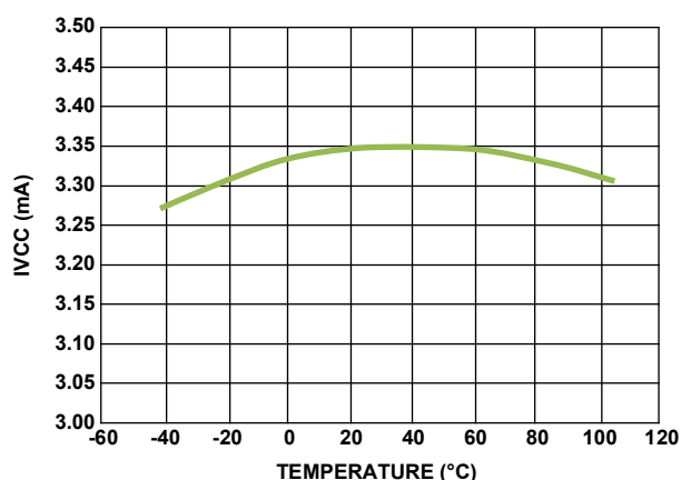
Figure 36. VCC Supply Current vs Temperature at 6V, 39.6V, 60V
