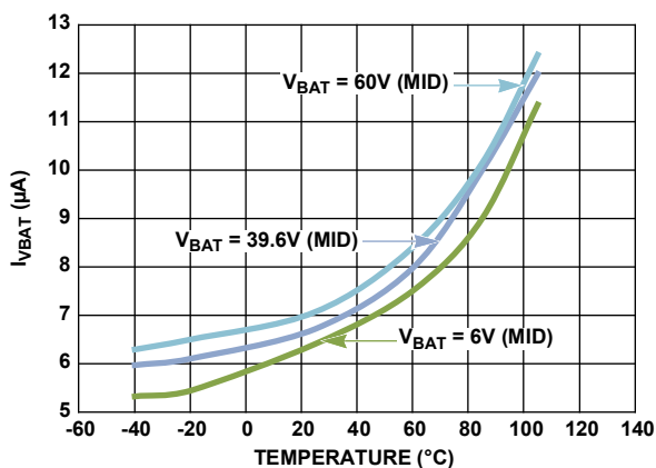
Figure 34. V_{BAT} Voltage Shutdown Current vs Temperature (EN = 0) AT 6V, 39.6V, 60V
