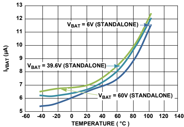
Figure 32. Pack Voltage Shutdown Current vs Temperature (EN = 0) at 6V, 39.6V, 60V
