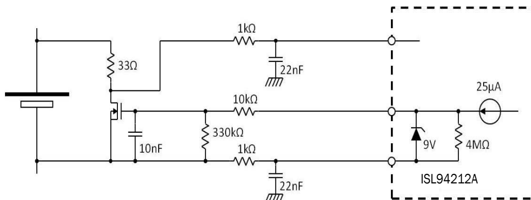
Figure 84. Balance Circuit Arrangement
