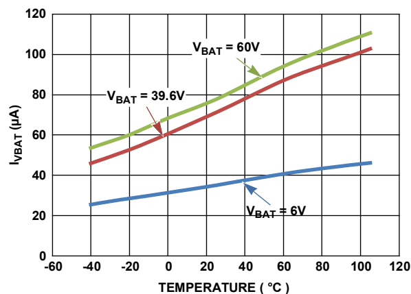
Figure 28. Pack Voltage Supply Current vs Temperature at 6V, 39.6V, 60V (Standalone Mode)
