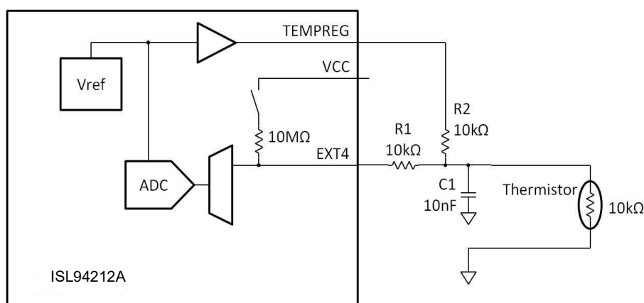
Figure 87. Connection of NTC Thermistor to Input EXT4
