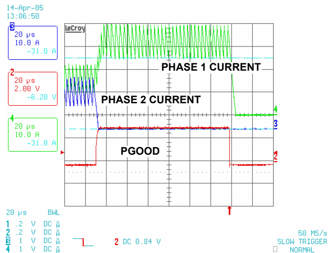
FIGURE 34. ISL9506, OVERCURRENT DUE TO PHASE DROPPING
