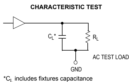
Figure 2. TTL Output Loading Used for Device Evaluation
