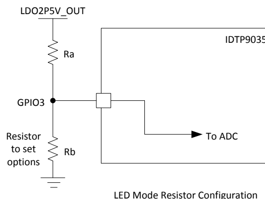
Figure 10. IDTP9035 LED Resistor Options.
