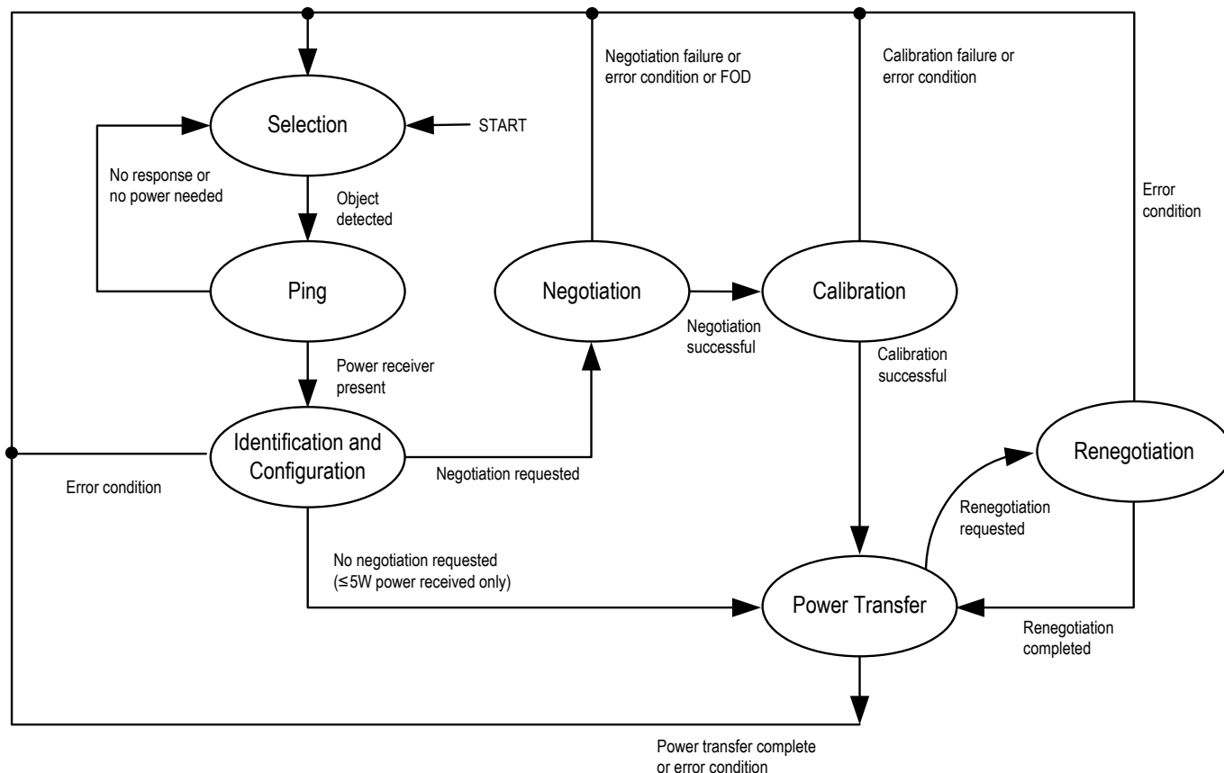
Figure 27. WPC Power Transfer Phases Flowchart
