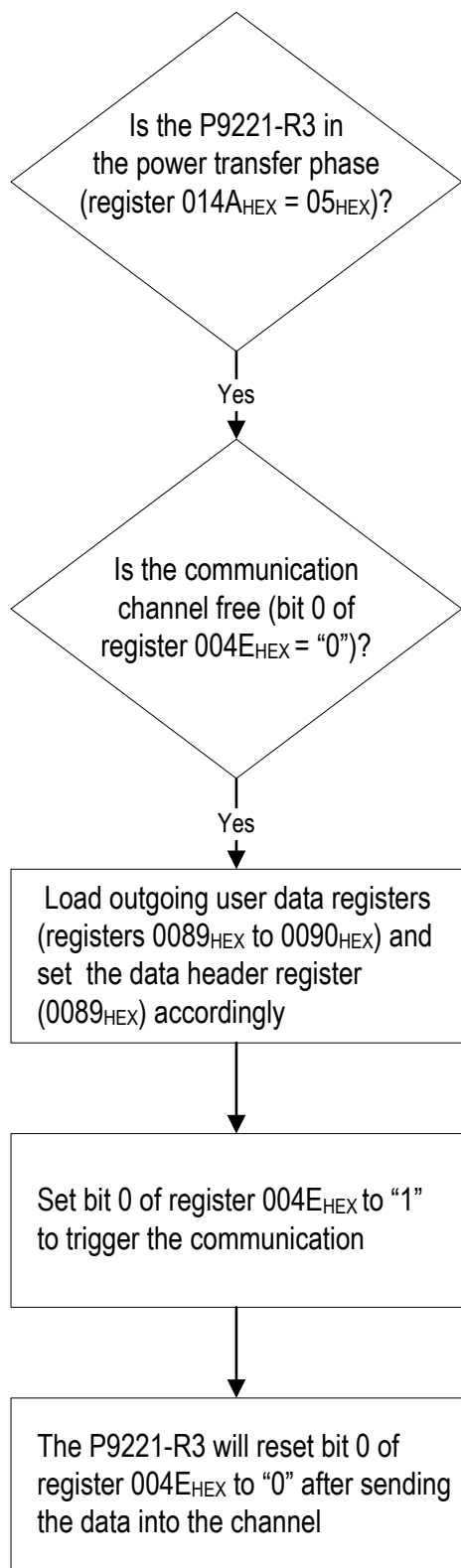
Figure 25. State Diagram for User Data Transmission from the P9221-R3 to the P9242-R3
