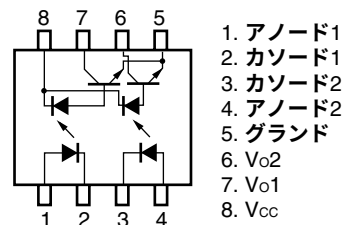
PS8821-2
