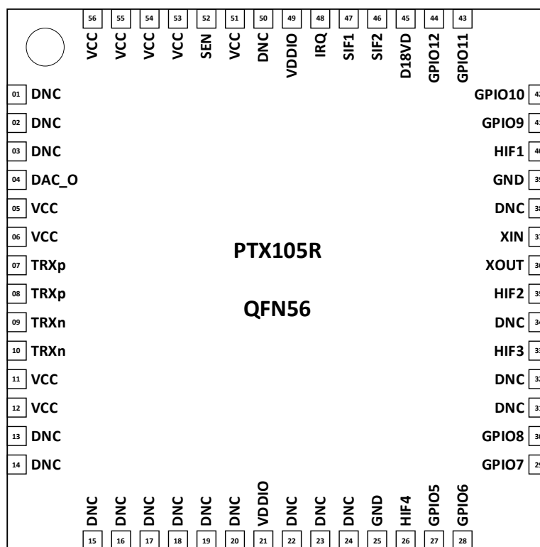
Figure 2: Pin Diagram
