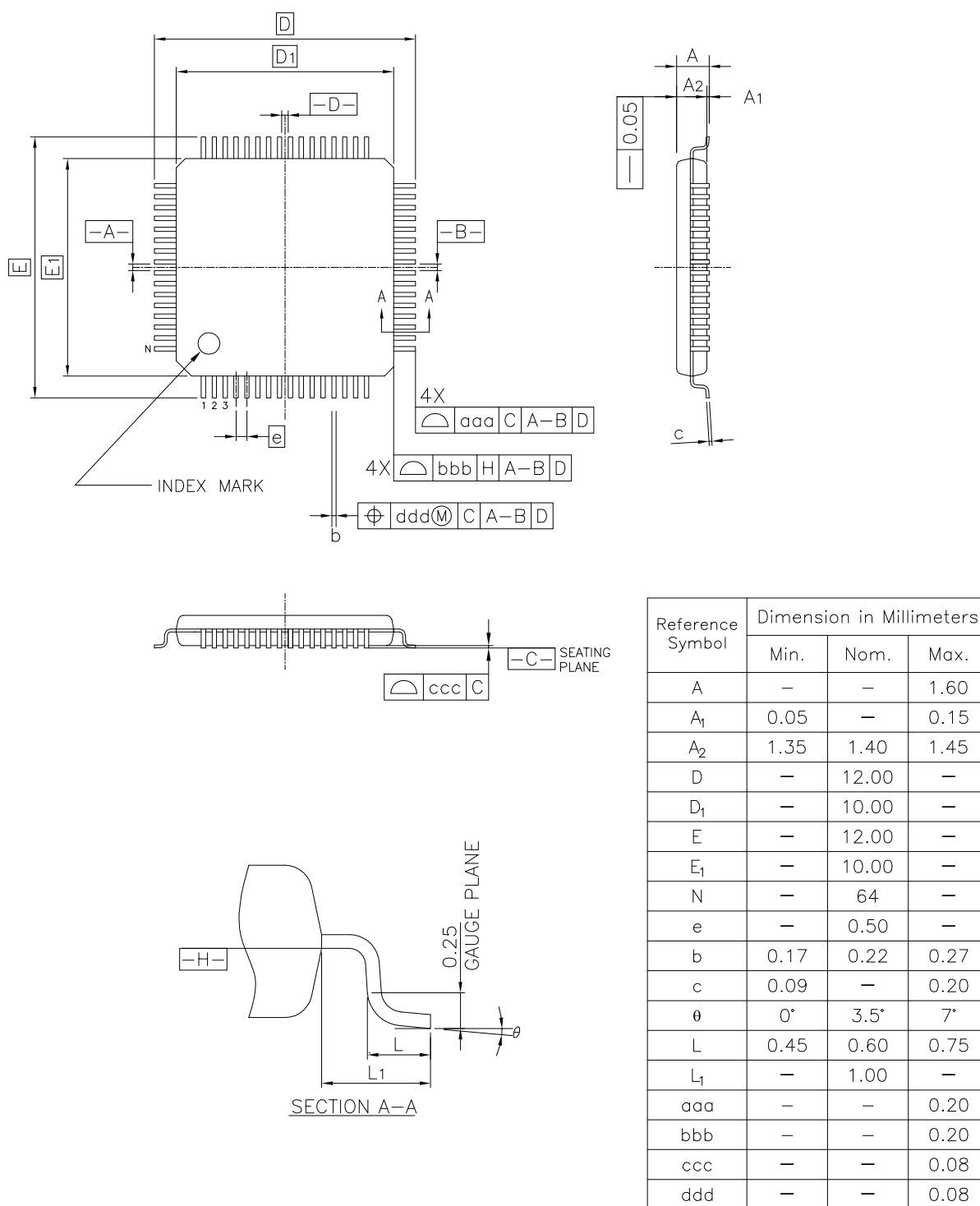
Figure A2.2 LQFP 64-pin 0.5mm pitch (2)
