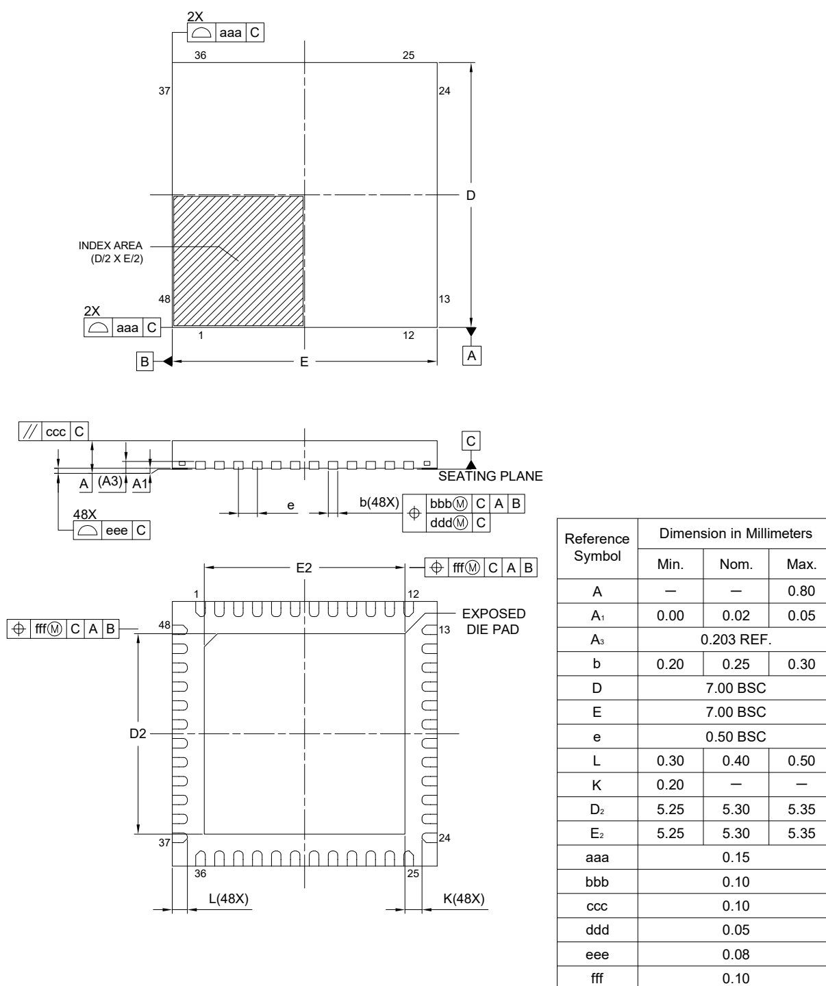
Figure A2.6 HWQFN 48-pin
