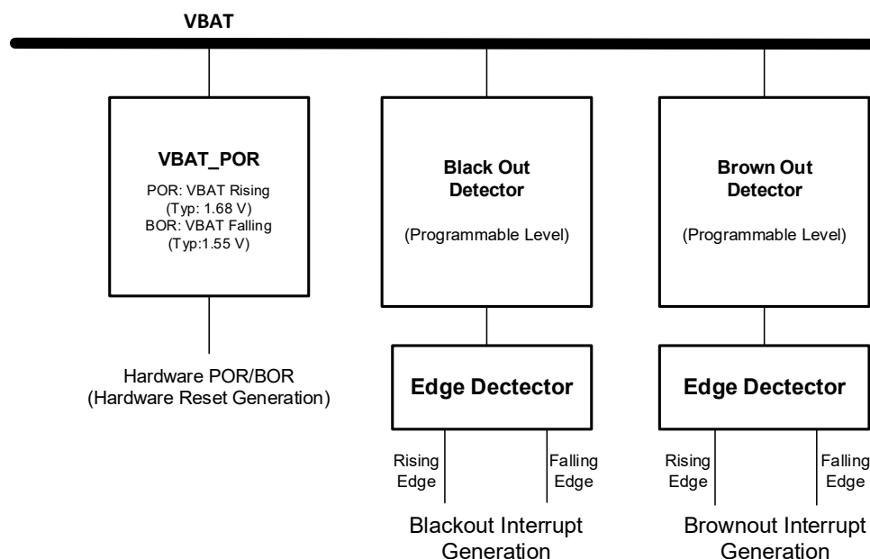
Figure 17. VBAT and POR, blackout/brownout detector
