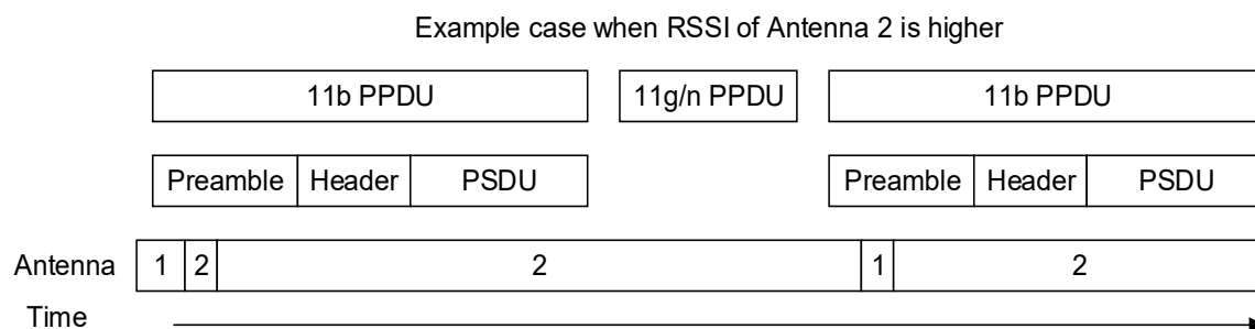
Figure 60. Antenna switching timing diagram
