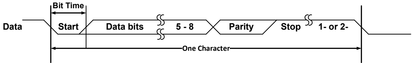
Figure 20. Serial data format
