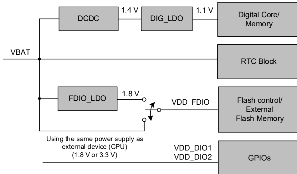
Figure 11. Power management block diagram
