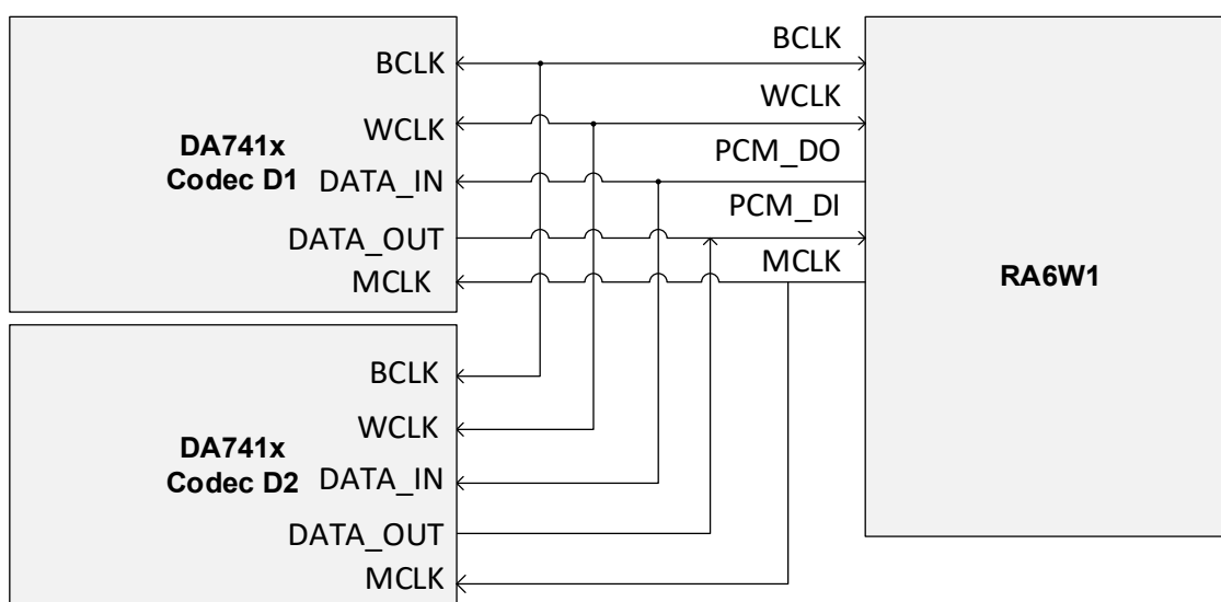
Figure 38. TDM configuration
