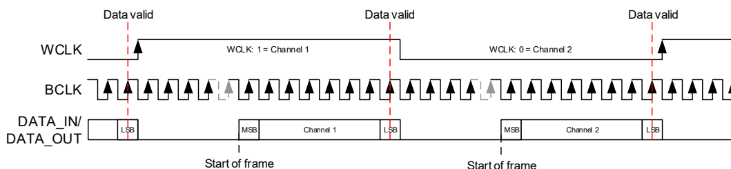
Figure 37. Right-justified format
