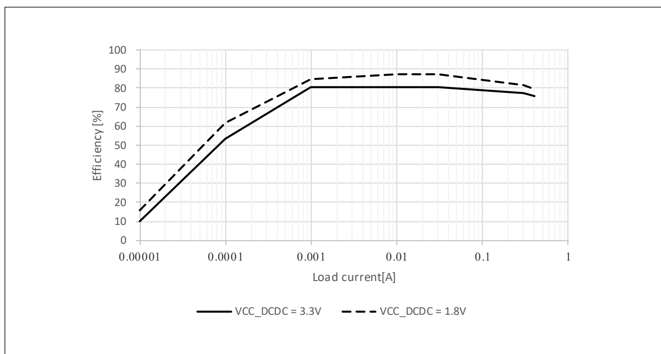
Figure 2.12 Typical DCDC efficiency (%) vs load current (A) in Low-speed mode and Software Standby mode, T_j = 125\text{ }^{\circ}\text{C}
