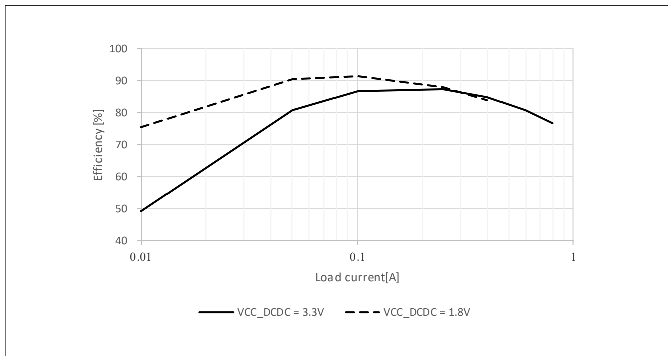
Figure 2.9 Typical DCDC efficiency (%) vs load current (A) in High-speed mode, T_j = 25\text{ }^{\circ}\text{C}
