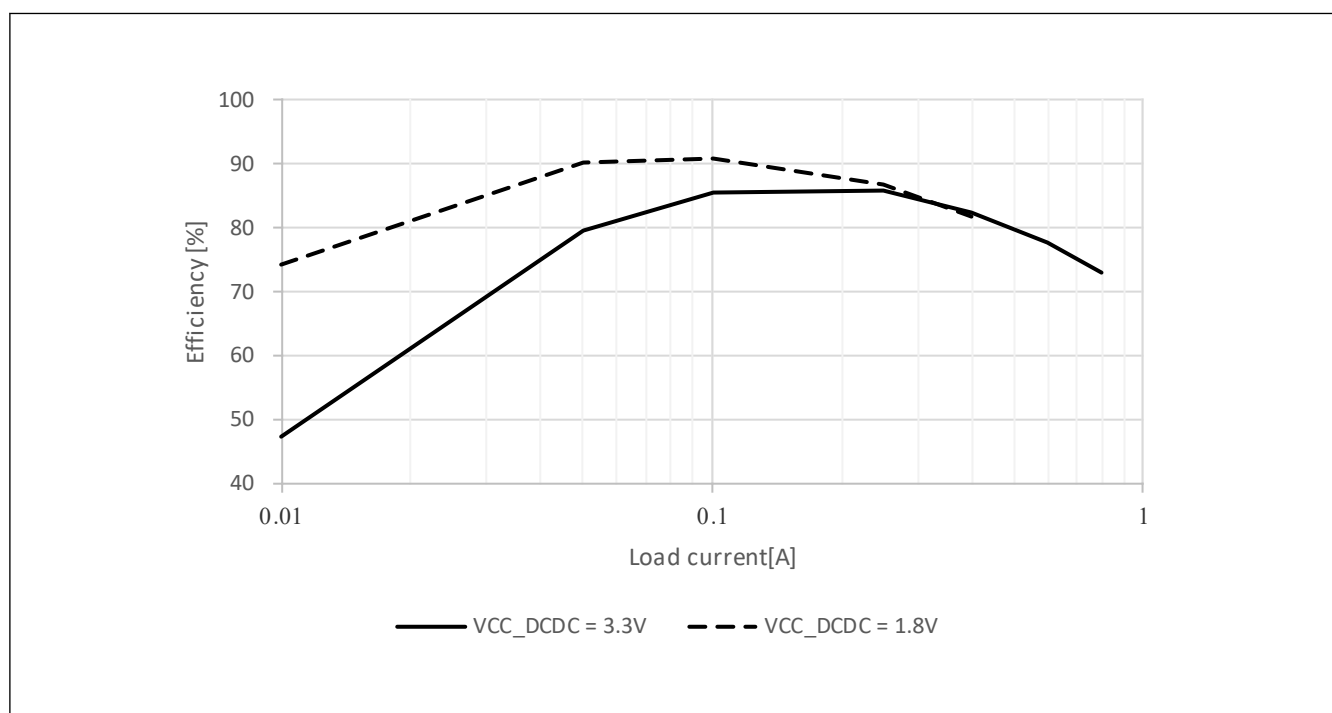
Figure 2.10 Typical DCDC efficiency (%) vs load current (A) in High-speed mode, T_j = 125\text{ }^{\circ}\text{C}
