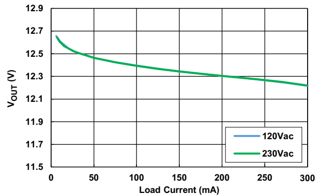
Figure 20. Load Regulation
