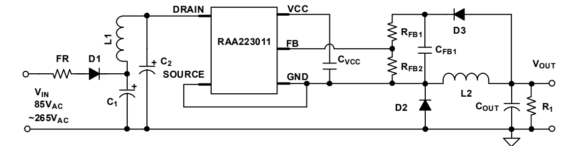
Figure 30. RAA223011 Buck with Low BOM Cost
