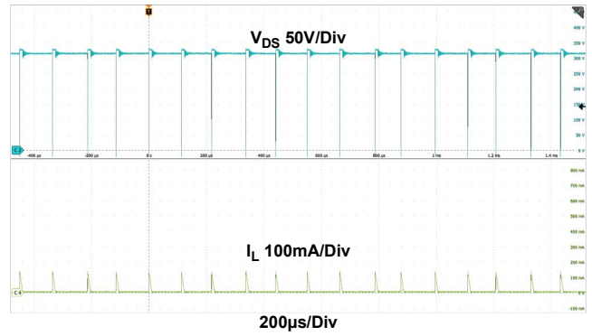
Figure 14. Light-Load Operation
