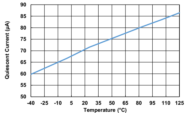
Figure 8. IC Quiescent Current vs Temperature
