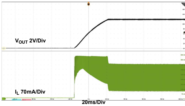
Figure 11. Startup
