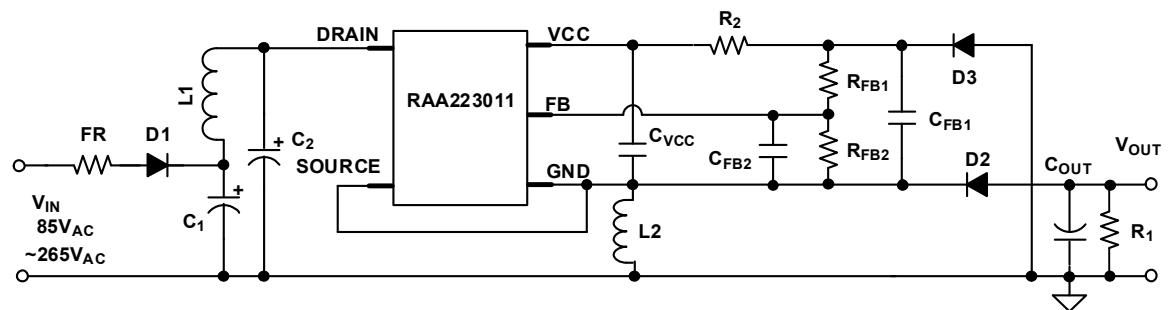
Figure 31. RAA223011 Buck/Boost
