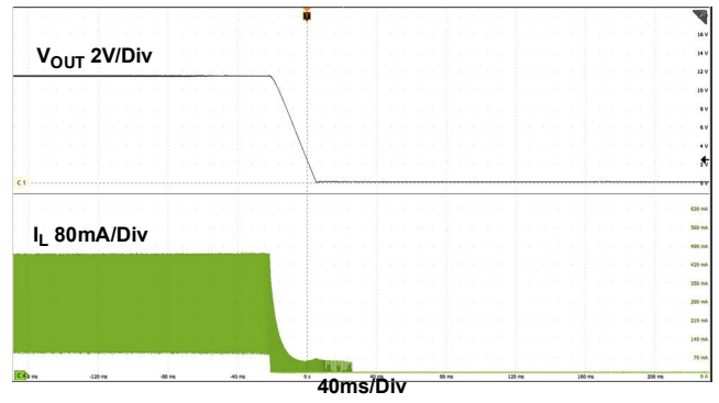
Figure 12. Shutdown
