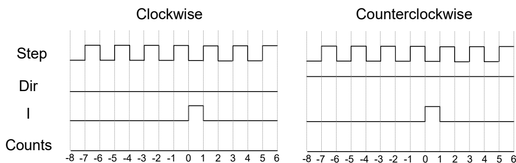
Figure 26. Step/Direction protocol
