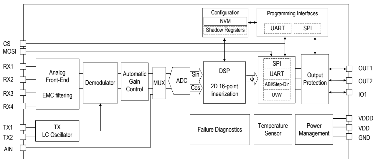
Figure 4. Block diagram
