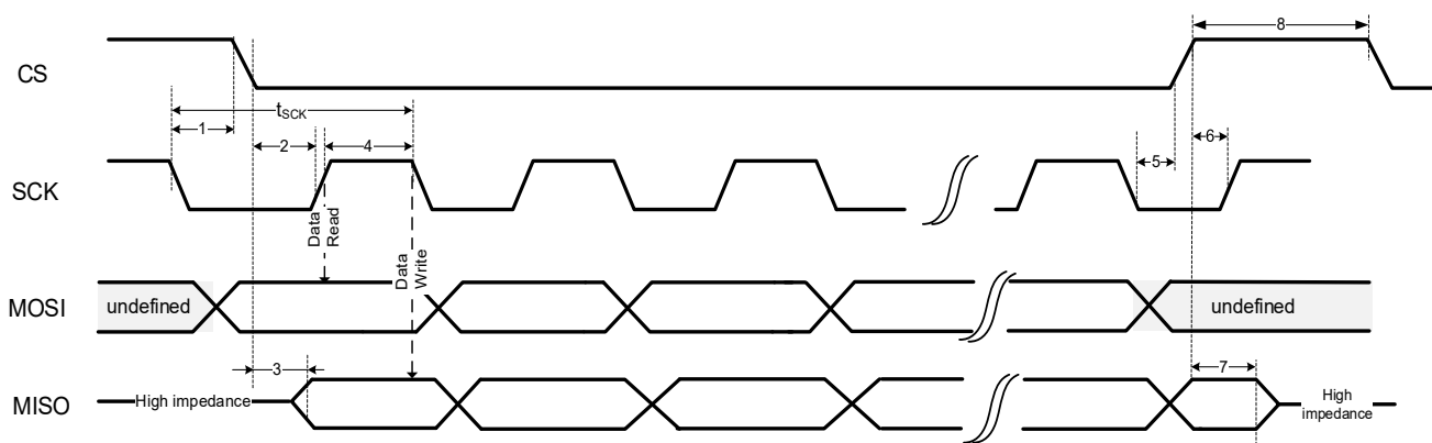
Figure 14. Safe SPI timing diagram for mode 0 (CPOL=0; CPHA=0)
