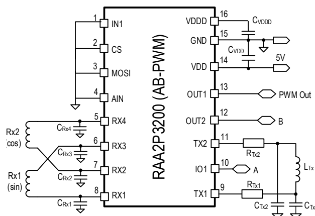
Figure 31. AB + PWM configuration
