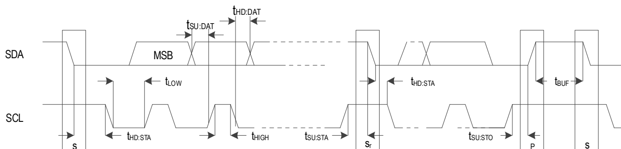
Figure 11. SMBus Target Timing Diagram
