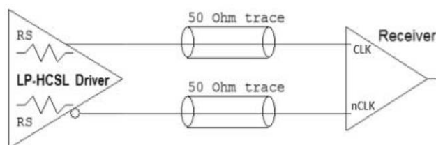
Figure 10. Standard LP-HCSL Termination
