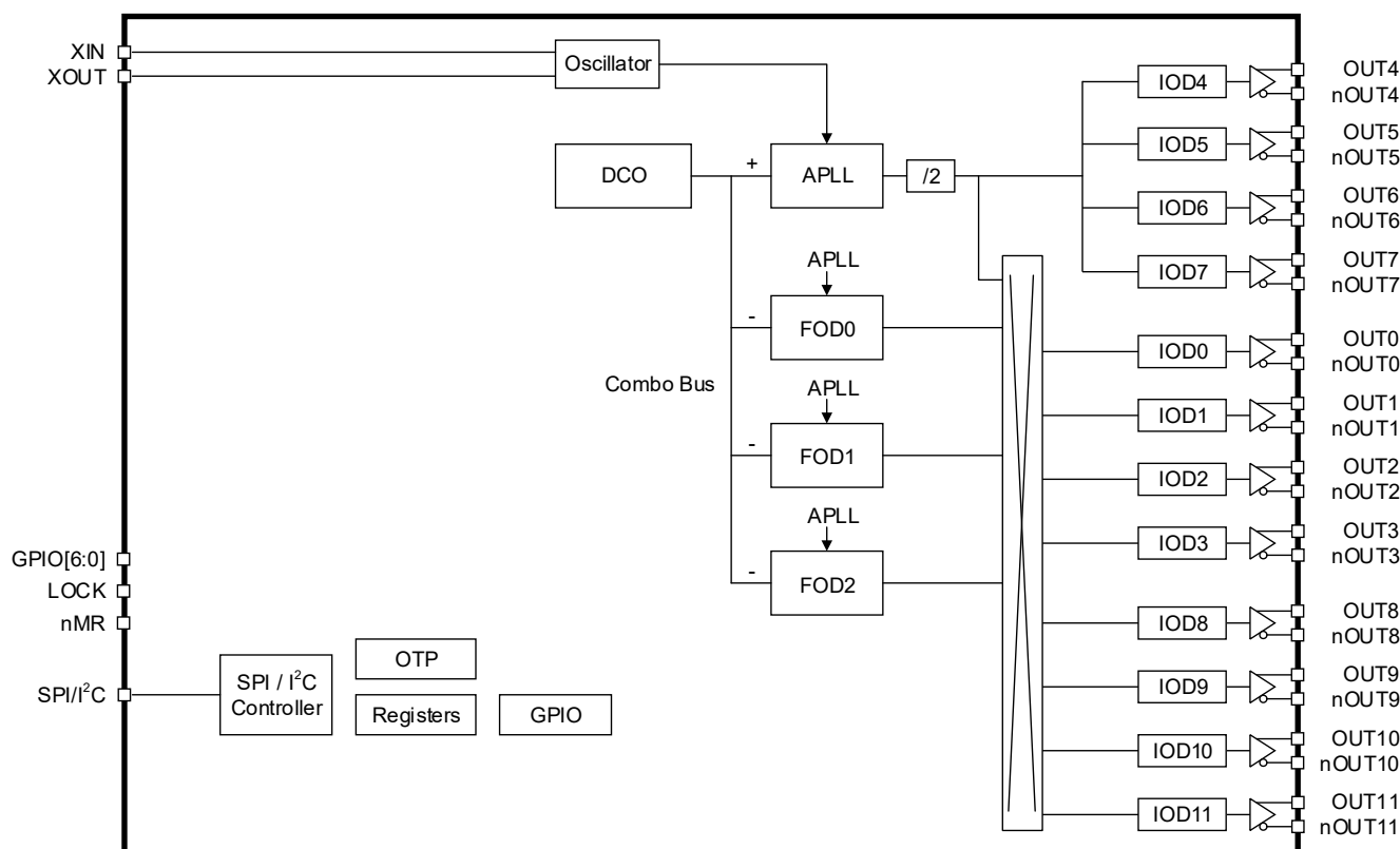
Figure 2. RC22312 Block Diagram
