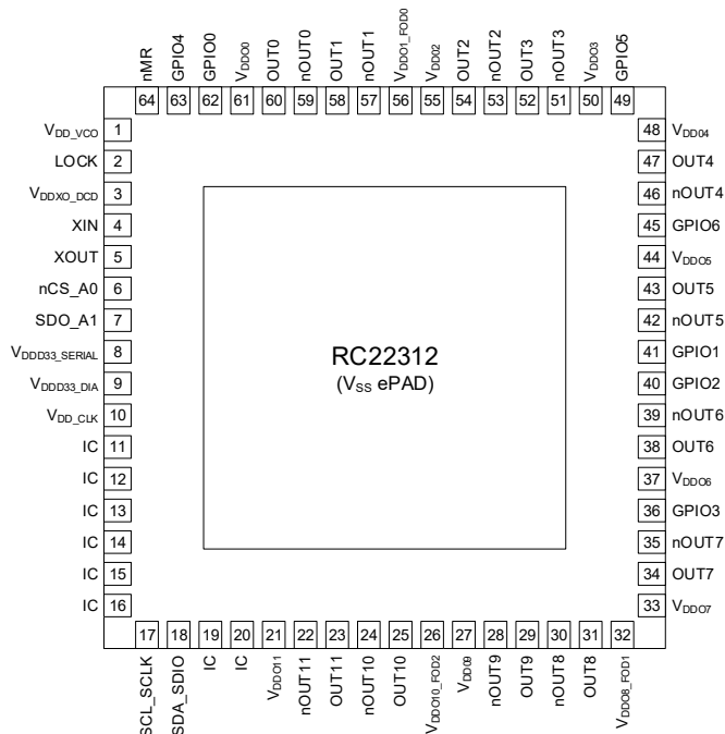
Top View (9 × 9 mm, 0.5mm lead pitch)
