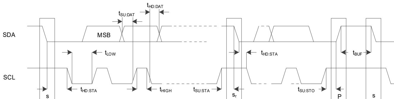
Figure 3. I²C Slave Timing Diagram
